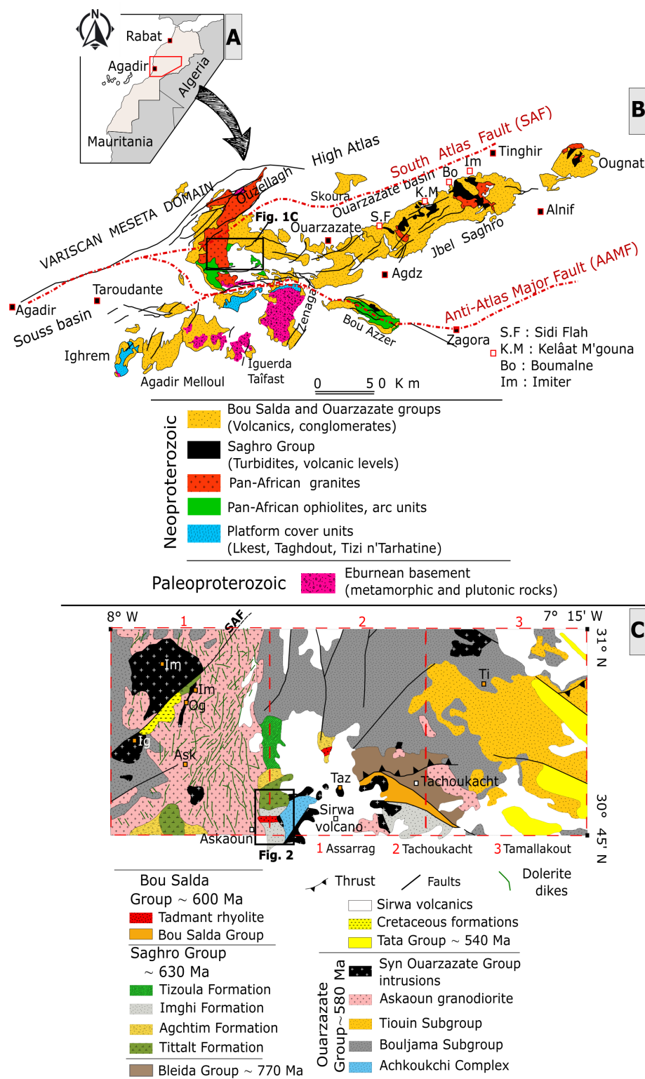
Figure 1. (A) Sketch map locating the Anti-Atlas belt in respect to Morocco (Saadi, 1985); (B) geological map of the Central and Eastern Anti-Atlas Proterozoic inliers (redrawn and modified after Michard et al. (2017)); (C) Schematic representation of the geology of the Sirwa massif (compiled and redrawn from Thomas et al. (2002); location of the ZGMR in Fig. 2. Abbreviations: Taz: Tazoult quartz-porphyry ( 559 \pm 6 Ma); Im: Imourkhsen granite ( 562 \pm 5 Ma); Ti: Tikhfist rhyolite ( 571 \pm 8 Ma); Ask: Askoun granodiorite ( 575 \pm 8 Ma); Ig: Ighrem granite; Og: Ougougane granite; and SAF: South Atlas Fault. U-Pb ages are from Thomas et al. (2002).
