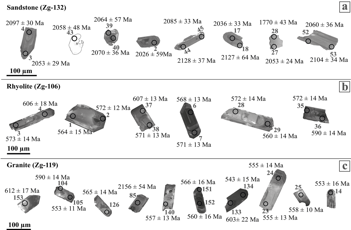
Figure 4. Cathodoluminescence (CL) images of representative zircon grains from the (a) SG sandstone (Zg-132); (b) OG rhyolite (Zg-106); and (c) OG granite (Zg-119). Black circles indicate analytical spots, with corresponding ^{206}\text{Pb}/^{238}\text{U} ages. The reported errors are 2 s.
