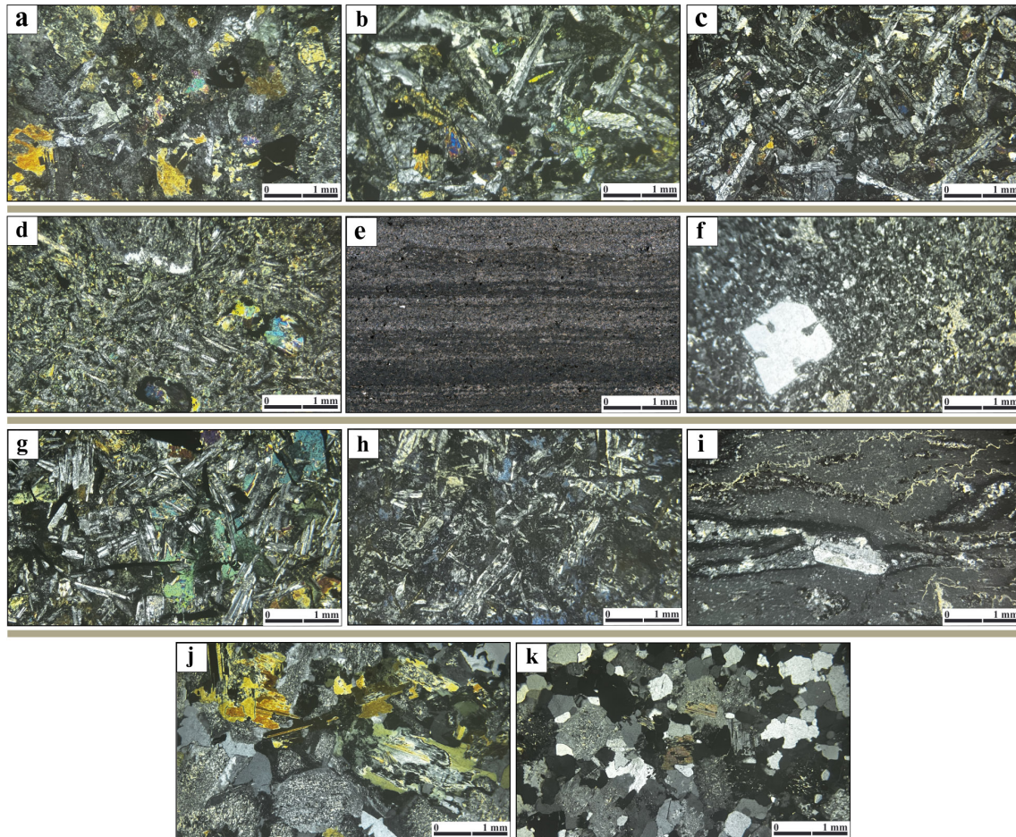
Figure 3. Photomicrographs (all in cross-polarized light) of the studied SG and OG rocks. (a) Gabbro sample showcasing a medium to coarse-grained locally equigranular texture; (b) An intergranular texture for dolerite; (c) Andesite showcasing an ophitic texture; (d) Microlitic-porphyritic texture for basaltic-andesite; (e) Sandstone (Zg-132) exhibiting millimetre-scale laminations showcasing darker bands enriched in chlorite, with quartz-muscovite lighter laminations; (f) Microcrystalline texture for rhyolite with embayed quartz phenocrysts; (g) Dolerite exhibiting an intergranular texture; (h) Diabase characterized by an intergranular texture with patches of blue chlorite; (i) Welded ignimbrite with an eutaxitic texture displaying flow textures with feldspars (sanidine) crystals embedded in a glassy fiamme; (j) Quartz diorite with subhedral to anhedral amphiboles and sericitized plagioclase; (k) Medium to locally fine-grained granite, with an anhedral to subhedral equigranular texture.
