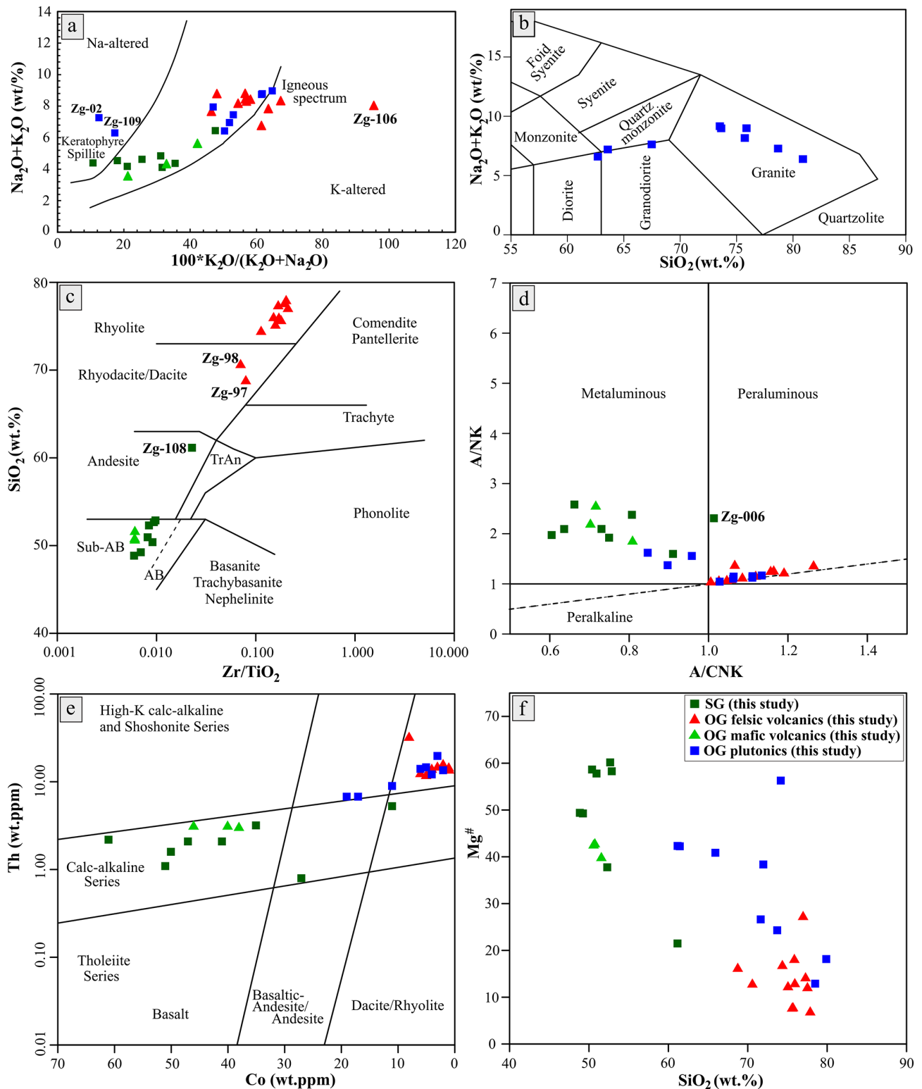
Figure 6. (a) \text{Na}_2\text{O} + \text{K}_2\text{O} (wt.%) versus 100 \times \text{K}_2\text{O}/(\text{K}_2\text{O} + \text{Na}_2\text{O}) plot of Hughes (1972); (b) TAS diagram (after Middlemost, 1994); (c) \text{SiO}_2 (wt.%) versus \text{Zr}/\text{TiO}_2 (Winchester and Floyd, 1977); (d) Plot of \text{A}/\text{NK} versus \text{A}/\text{CNK} ( \text{A}/\text{CNK} = molar ratio \text{Al}_2\text{O}_3/(\text{CaO} + \text{Na}_2\text{O} + \text{K}_2\text{O}) and \text{A}/\text{NK} = molar ratio \text{Al}_2\text{O}_3/(\text{Na}_2\text{O} + \text{K}_2\text{O}) ) (Shand, 1943); (e) Plot of \text{Th} (ppm) versus \text{Co} (ppm) of Hastie et al. (2007); (f) \text{Mg}^\# value versus \text{SiO}_2 contents (wt.%).
