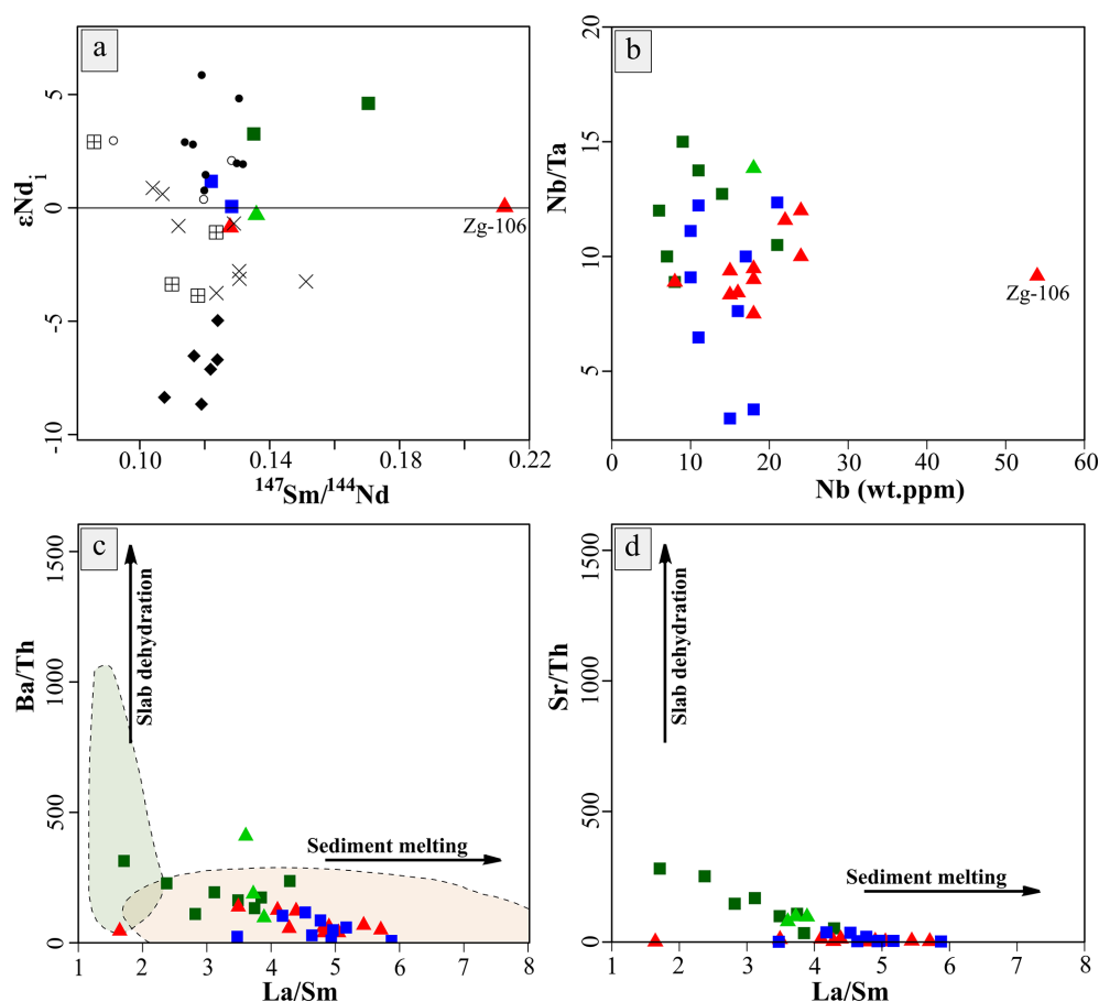
Figure 10. Plots (a) Initial \epsilon\text{Nd}_1 versus ^{147}\text{Sm}/^{144}\text{Nd} ; (b) Nb/Ta versus Nb contents (ppm); (c) Ba/Th versus La/Sm and (d) Sr/Th versus La/Sm (domains are modified from Labanieh et al. (2012). Legend is the same as in Fig. 8.
