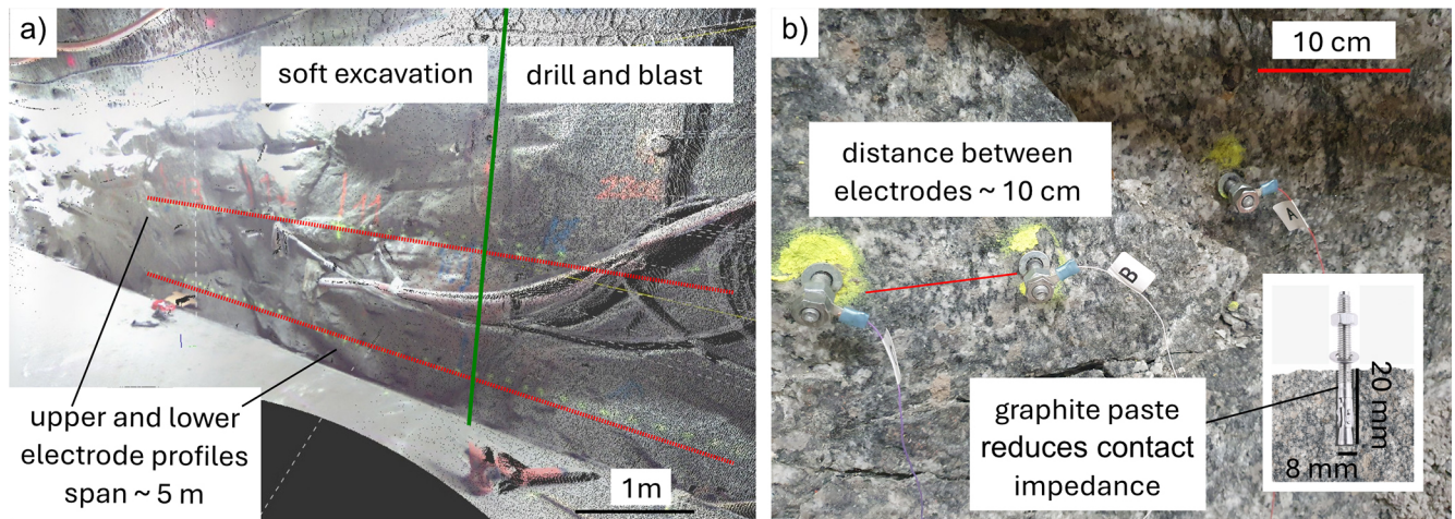
Figure 9. (a) Illustration of the electrical resistivity profiles installed on the tunnel wall, that transverse between soft excavation and drill-and-blast. The image is derived from a laser scan (ref) and shows the roughness of the tunnel wall. (b) A closeup picture of three electrodes, indicating the relevant dimensions and wall roughness.
