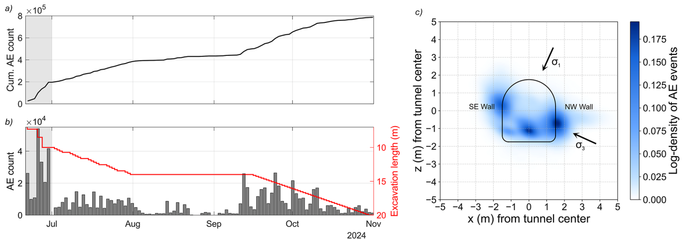
Figure 11. AE monitoring during PRECODE tunnel excavation: (a) cumulative AE count during PRECODE excavation (shaded area indicates drill and blast excavation); (b) AE count during PRECODE tunnel excavation with excavation lengths marked as red solid line; (c) Log-density of AE events registered during the PRECODE tunnel excavation in an x – z plane. The ideal tunnel geometry is marked for reference.
