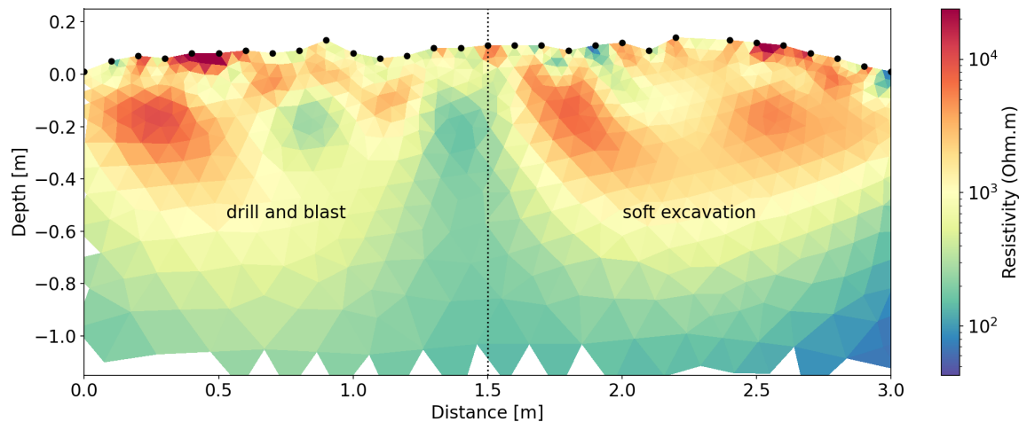
Figure 14. Inversion results for electrical resistivity tomography spanning the drill and blast, and soft excavation zones. The results show some prominent very high resistivity zones in the shallow few centimeters, likely resulting from loose slabs of rock along the wall. The information at depth reveals a higher resistivity zone for the soft excavation, suggesting more intact rock compared to the drill and blast zone.
