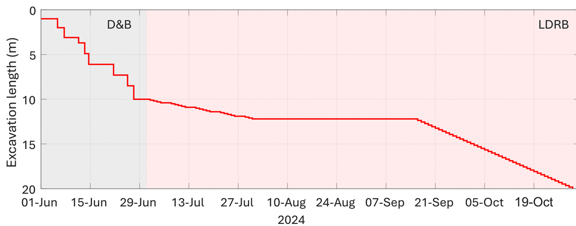
Figure 5. Excavation advancement for the PRECODE section.
