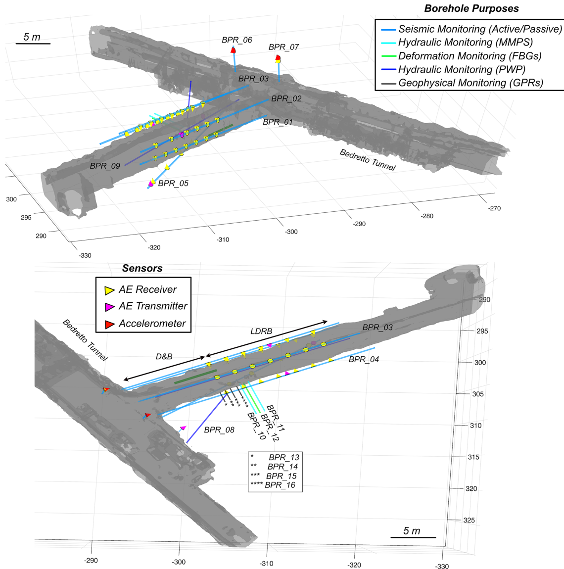
Figure 6. Multidisciplinary monitoring scheme of the PRECODE Section.
