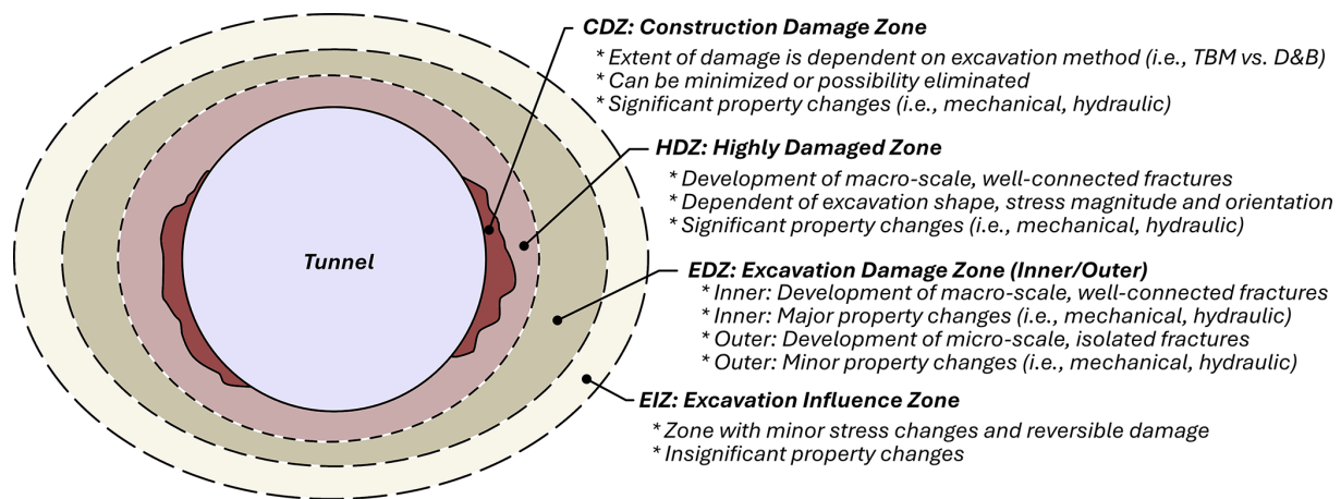
Figure 2. Definition of various damage zones around tunnels and their associated characteristics (modified after Siren et al., 2015; Perras and Diederichs, 2016).
