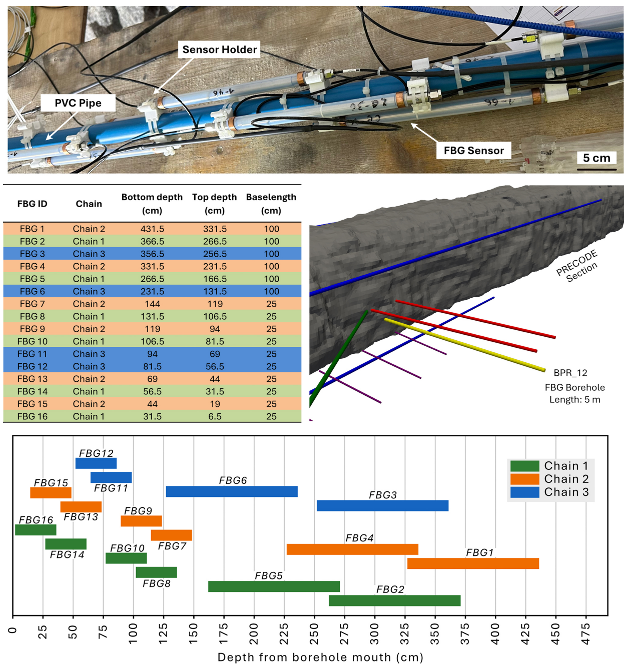
Figure 10. FBGs layout in BPR_12 borehole to monitor the development of deformation, Top: An example of the FBG array, Middle: list of installed FBGs and isometric view of the borehole, Bottom: schematic illustration of the installed FBG within the borehole and their overlaps.
