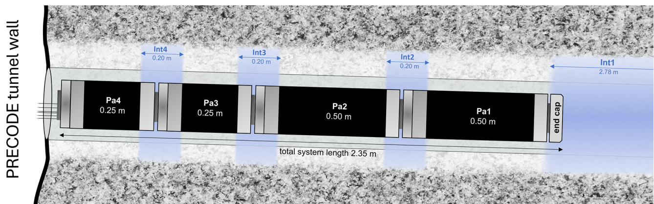
Figure 8. Schematic illustration of the modular multi-packer system (MMPS) installed in boreholes BPR_B_10 and BPR_B_11. The configuration is identical for both boreholes. Packer sleeve lengths (Pa1–Pa4) and the resulting hydraulically isolated test intervals (Int1–Int4).
