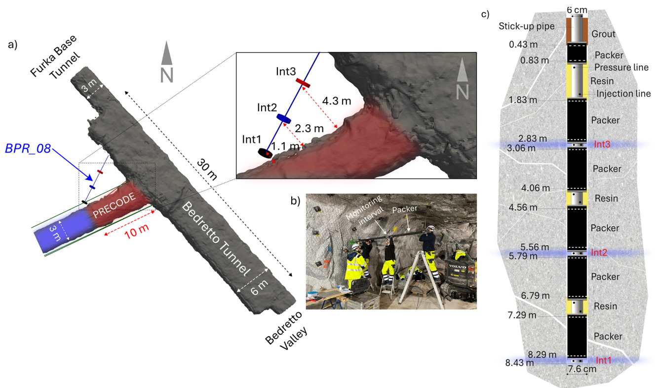
Figure 7. (a) Instrumentation of the BPR_08 pressure monitoring borehole during the PRECODE experiment; (b) an image of the packer system during installation, (c) the detail of the three monitoring intervals.
