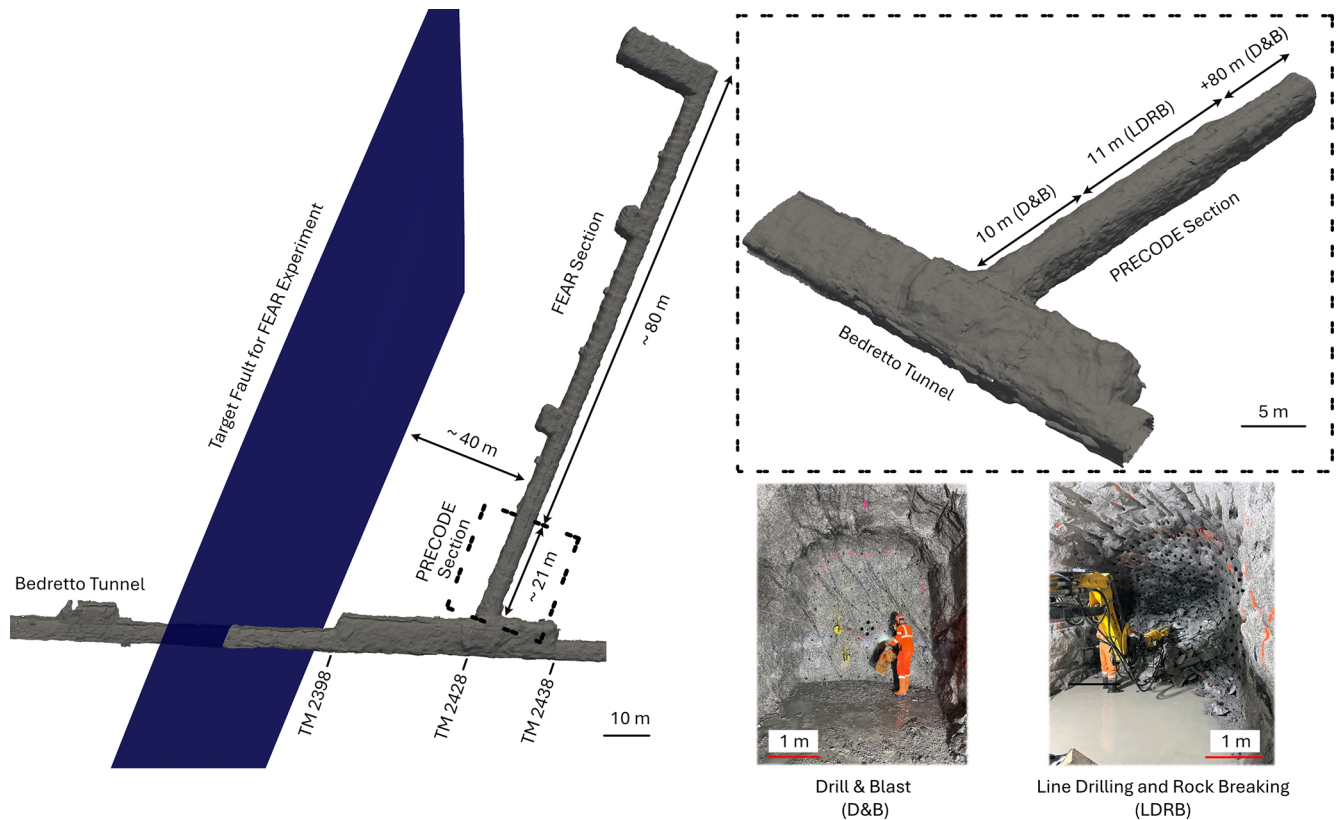
Figure 4. Left: Isometric view of the Bedretto Tunnel and the newly-excavated PRECODE/FEAR Tunnel, Right: As-built geometry of the PRECODE Section, showing D&B and LDRB sections.
