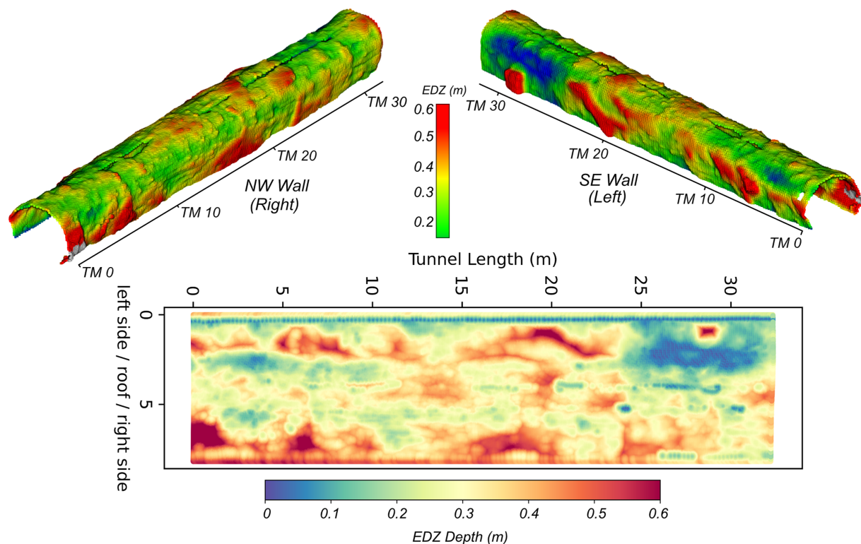
Figure 12. The calculated depth of EDZ around the PRECODE Tunnel obtained from TLS, Top: Isometric view of the EDZ depth on the 3D point clouds, Bottom: EDZ depth projected on the unwrapped PRECODE tunnel.
