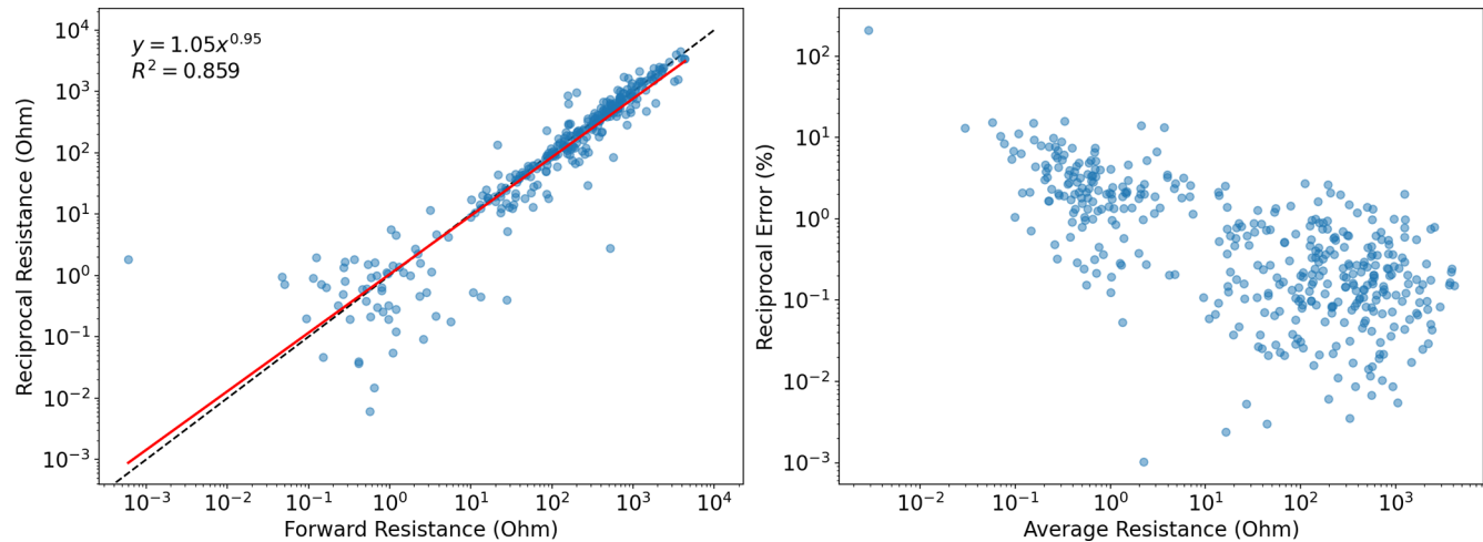
Figure 13. The left panel shows a comparison of forward and reciprocal electrical resistivity measurements for the profile under examination, alongside the perfect match line. The forward and reciprocal measurements overlap well, especially for high resistivities, suggesting high precision. The right panel shows the reciprocal error compared to the average resistance for the measurements. Reciprocal errors above 10 % are not included in the data inversion.
