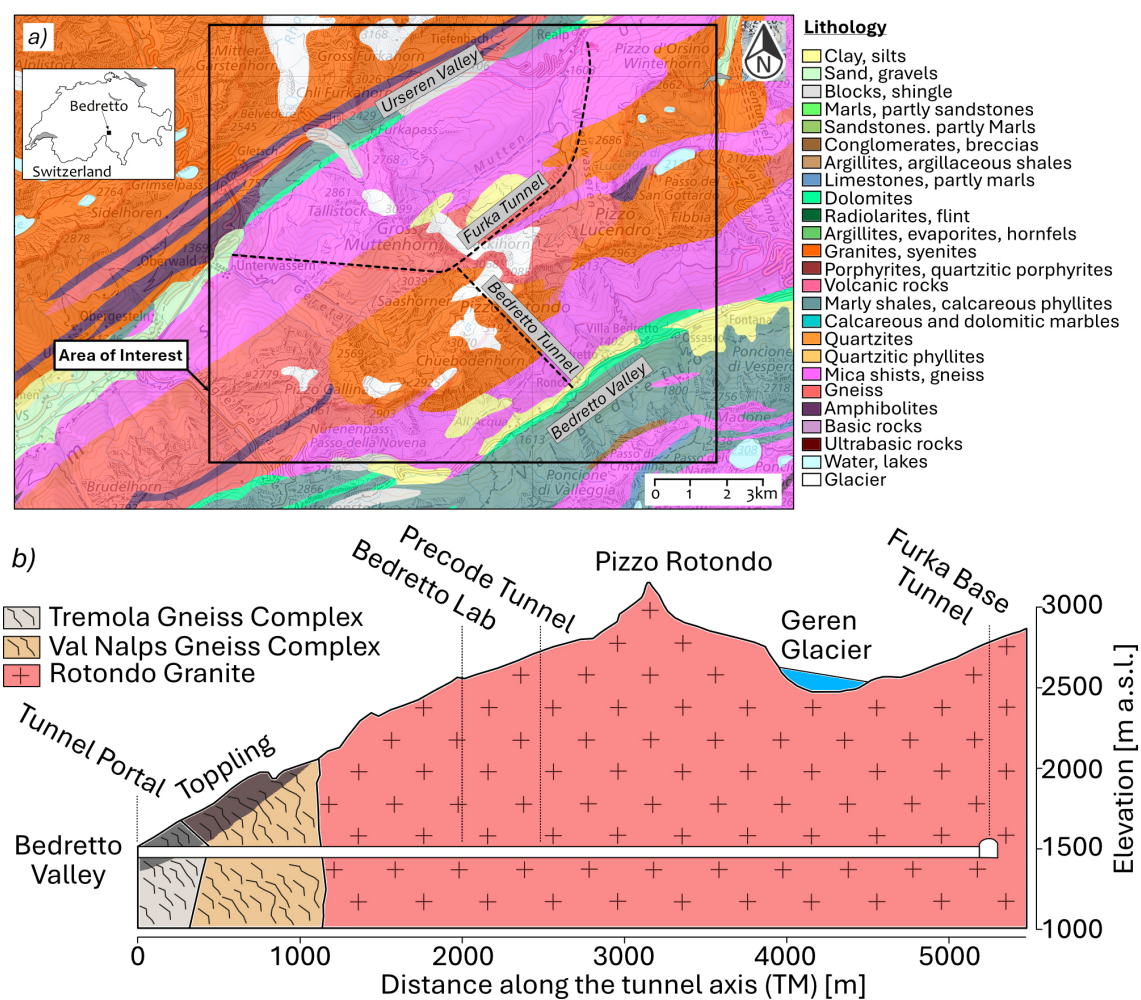
Figure 3. (a) Lithology of the Bedretto Valley (source: SwissTopo), (b) cross section along Bedretto Tunnel, with highlighted location of BedrettoLab and PRECODE Tunnel (modified after Keller and Schneider, 1982).
