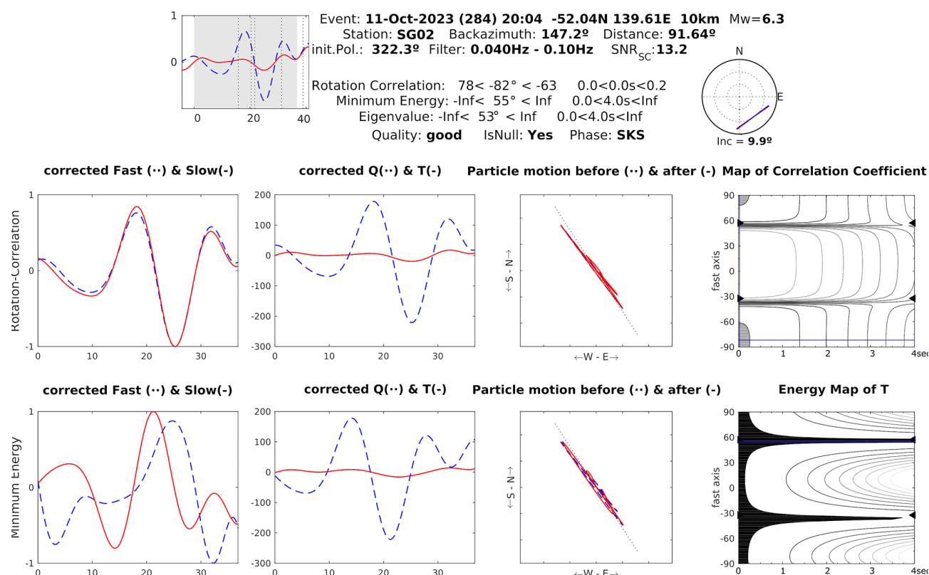
Figure 6. An example of null measurement at SG02 seismic station. For the description, see Fig. 4.
