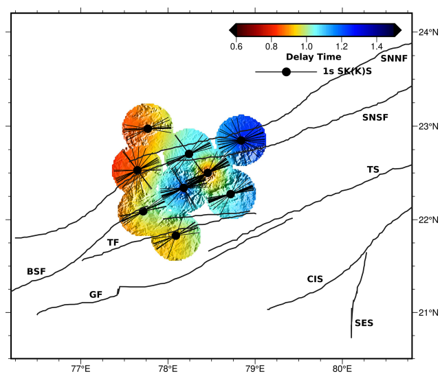
Figure 8. The FPD and delay times of individual SK(K)S splitting measurements at each seismic station. The azimuth of the black bars denotes the individual FPDs of the obtained splitting parameters. The interpolated station-averaged split delay time at each seismic station is presented in a color-coded format to illustrate lateral variations in delay times. The black circles indicate the seismic stations used in this study.
