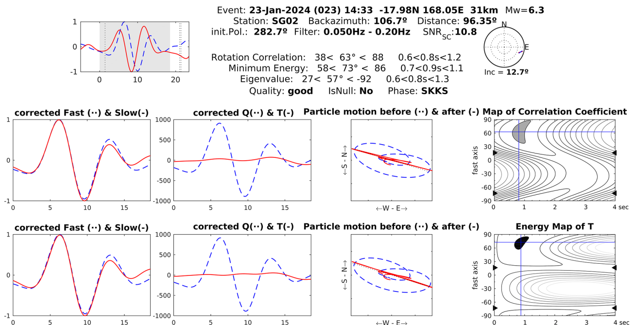
Figure 5. An instance of good SKKS-derived splitting measurement for an event recorded by the SG02 seismic station. For the description, see Fig. 4.
