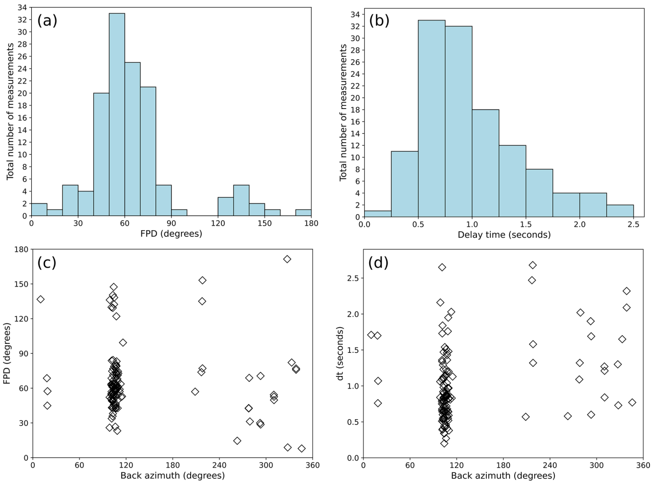
Figure 7. Histograms illustrating individual splitting parameters: (a) fast polarization directions (FPDs) and (b) delay times ( \delta t ). (c) and (d) illustrate the back azimuthal variation of individual FPDs and \delta t s across all seismic stations, respectively. The majority of splitting measurements are concentrated within the backazimuthal range of 90 to 120°.
