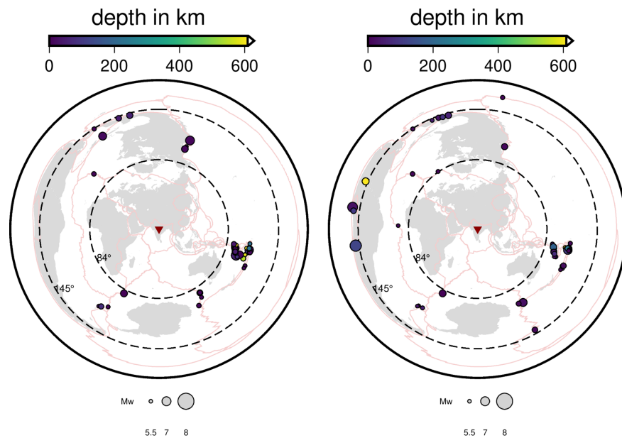
Figure 3. The epicentral distribution of earthquake events for (a) SKS (84–145°) and (b) SKKS (84–180°) seismic phases. The inverted dark red triangle represents the central location of seismic stations, while the circles denote earthquake events. The variation in circle colour indicates the depth of the earthquake events, while the size differences correspond to their magnitude.
