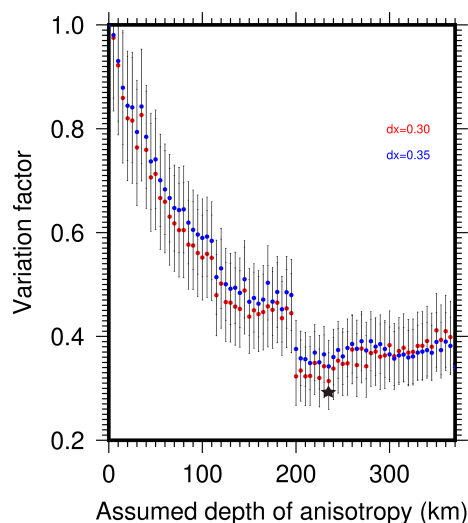
Figure 11. Depiction of the variation factor as a function of the presumed depth of anisotropy, calculated for block sizes of 0.30 and 0.35°. The variation factor is calculated as the weighted sum of the circular mean of the fast polarization directions and the arithmetic mean of the delay times.
