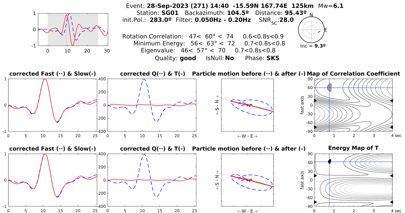
Figure 4. An example of a good SKS splitting phase for an earthquake recorded by the SG01 seismic station. The upper left graphic displays the radial component (blue dotted) and transverse (red solid) component, with the chosen time frame highlighted in gray. The top bar displays the event, station, and computed result information simultaneously. The stereoplot is shown in the top right corner. The second row presents the outcomes of the rotation-correlation (RC) method, including SKS fast directions (blue dashed) and slow ones (red solid) after RC delay correction; radial (blue dashed, Q) and transverse (red solid, T) components after RC delay correction; particle motion before (blue dashed) and after (red solid) RC delay correction; and a map of correlation coefficients. The third row displays the results of the transverse energy minimization technique. The descriptions are similar to the RC plots.
