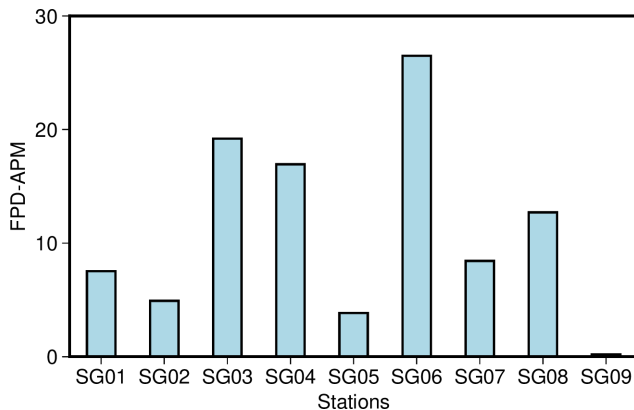
Figure 10. The bar diagram depicts the absolute difference between the station-averaged FPD for each station and the APM direction of the Indian plate, signifying the deviation of FPDs from the APM direction.
