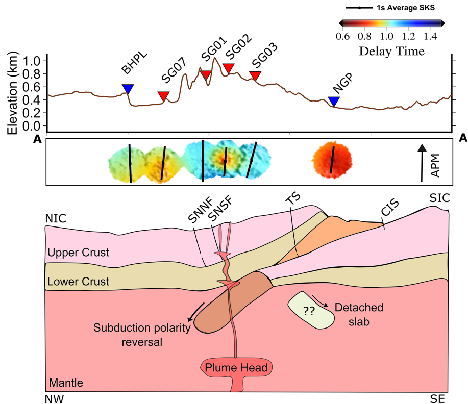
Figure 12. A hypothetical model (not to scale) depicting all tectonic events that have influenced the formation of CITZ over time and affected the FPD alignment and \delta t s. The model is built along AA' profile, extending from a low deformation area in the northwest to an active subduction zone in the southeast, as illustrated in Fig. 11. The elevation profile at the top illustrates the present-day topography along the A-A' transect, showing seismic station locations from the present study (red triangles) and previous studies (blue triangles). The middle panel denotes the average splitting measurements; bar length is proportional to delay times, and orientation indicates fast polarisation directions along with the interpolated split delay time at each station, which is displayed in a color-coded style to distinctly illustrate lateral variations in split delay times. The schematic cross-section in the bottom panel depicts the Mesoproterozoic collisional era ( \sim 1.55 – 0.85 Ga), specifically capturing the subduction polarity reversal and N-directed subduction of the SIC and possible subduction polarity reversal, as well as mantle plume activity during the late Cretaceous to early Paleocene. The subduction model representing the Mesoproterozoic collisional stage ( \sim 1.55 – 1.10 Ga) is modified from Deshmukh and Prabhakar (2020) and Mall et al. (2008), while the plume upwelling is additionally demonstrated by Shukla et al. (2022). APM: Absolute Plate Motion, NIC: North Indian Craton, SIC: South Indian Craton.
