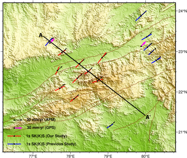
Figure 9. Lateral variation of the anisotropic and geodetic data illustrated on the tectonic and topographic map of the study region. The station-averaged splitting measurements for this study are depicted in red, whereas previous splitting measurements in adjacent regions are represented in blue. The black dots signify the location of the stations. The inclination of each bar represents the FPD, while the length denotes the \delta t . The GPS velocity vectors are depicted in magenta, whereas the APM direction of the Indian plate at each seismic station is represented in black.
