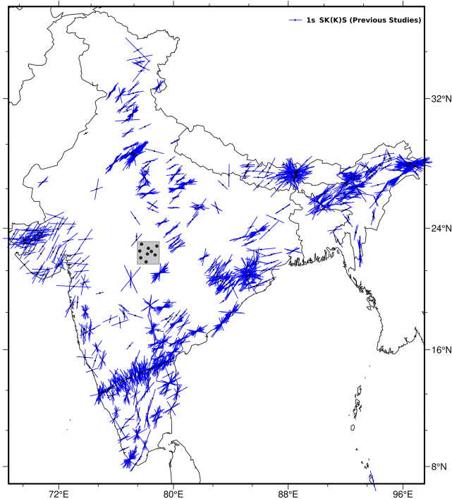
Figure 2. The figure illustrates the earlier SK(K)S-derived seismic anisotropy for the Indian region, depicted in blue ( http://ds.iris.edu/spud/swsmeasurement , last access: 20 September 2026), alongside our seismic stations, indicated in black circles. The bar length representing data at each seismic station corresponds to the \delta t s, while their orientation indicates the FPDs. IRIS Data Services data courtesy of IRIS.
