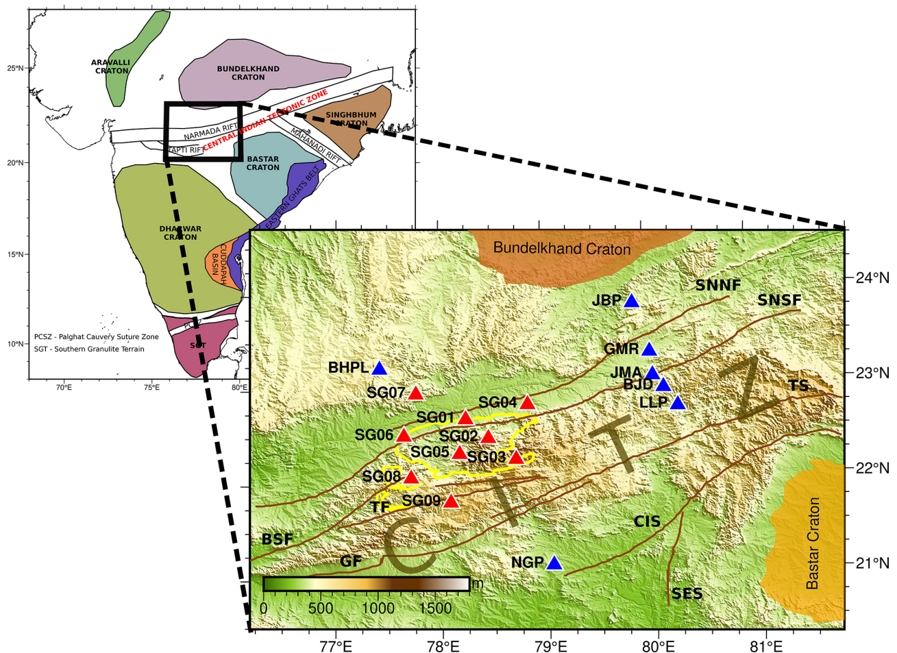
Figure 1. Tectonic and topographic map of the Central Indian Tectonic Zone across the Satpura Gondwana Basin. Red triangles denote the temporary seismic stations installed in and around the Satpura Gondwana Basin, whereas blue triangles indicate the seismic stations reported by Roy et al. (2014) and Roy et al. (2024). The fault lines shown in brown and the yellow curved lines denoting the boundary of the Satpura Gondwana Basin are adopted from Singh et al. (2015). Top Left: Regional geological and tectonic setting of Peninsular India, highlighting the distribution of Archean cratonic blocks and Proterozoic mobile belts (modified after Groves and Santosh, 2021). BSF: Barwani Sukta Fault; CIS: Central Indian Suture; GF: Gavligarh Fault; SNNF: Son Narmada North Fault; SNSF: Son Narmada South Fault; TF: Tapti Fault; TS: Tan Shear; SES: Sakoli East Shear.
