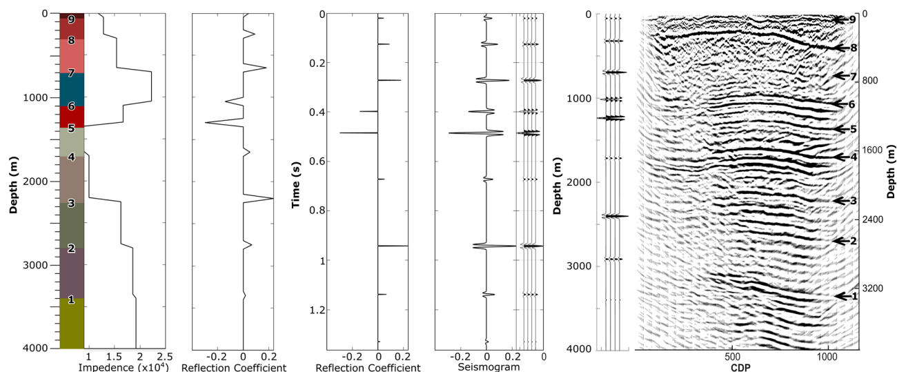
Figure 9. One-dimensional (1D) synthetic seismogram generated using average physical properties derived from interpreted geological contacts on the seismic profiles, as well as profile 1 showing key reflection contacts numbered 1 to 9 from bottom to top and correspond to: (1) the Ventersdorp Supergroup – Campbellrand and Schmidtsdrif Subgroup contact; (2) Campbellrand and Schmidtsdrif – Asbestos Hills and Koegas Subgroup contact; (3) the boundary between the Ghaap and Postmasburg Groups; (4) the Makganyene–Ongeluk Formation contact; (5) the Ongeluk–Hotazel Formation contact; (6) the Hotazel–Moodraai Formation contact; (7) the pre-Gamagara unconformity between the Transvaal and Keis Supergroups; (8) the Keis–Karoo Supergroup contact; and (9) the surface unconformity between the Karoo Supergroup and the overlying Kalahari Group.
