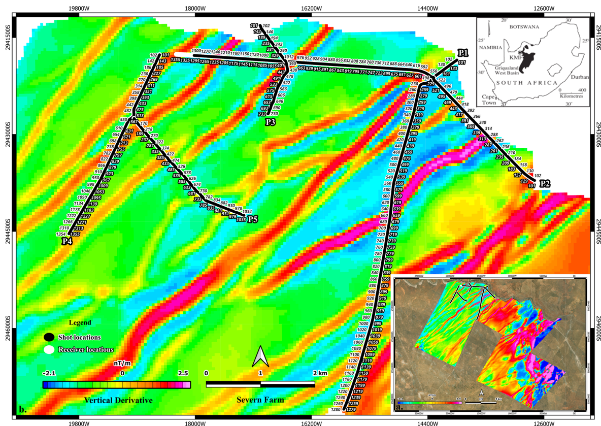
Figure 2. Seismic acquisition layout in relation to magnetic anomalies across the Kalahari Manganese Field (KMF). (a) First vertical derivative (1VD) of the Total Magnetic Intensity (TMI) map with 2D reflection seismic profiles overlain, illustrating the correlation between subsurface magnetic structures and the seismic survey lines. (b) Zoomed-in view of the Severn farm area showing the detailed layout of the 2D seismic profiles with shot and receiver positions superimposed on the magnetic map. The map highlights localized magnetic anomalies associated with subsurface lithological contrasts relevant to manganese exploration.
