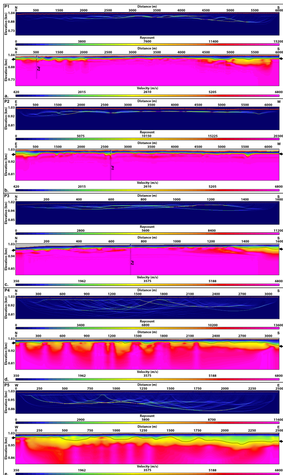
Figure 6. Refraction tomographic P-wave velocity models with associated ray coverage for seismic profiles 1 to 5 (a–e, respectively). The models display near-surface velocity variations, with velocities ranging from 600 to 5500 m s -1 . The base of the Kalahari Group sediments is interpreted and indicated by black arrows and dotted lines.
