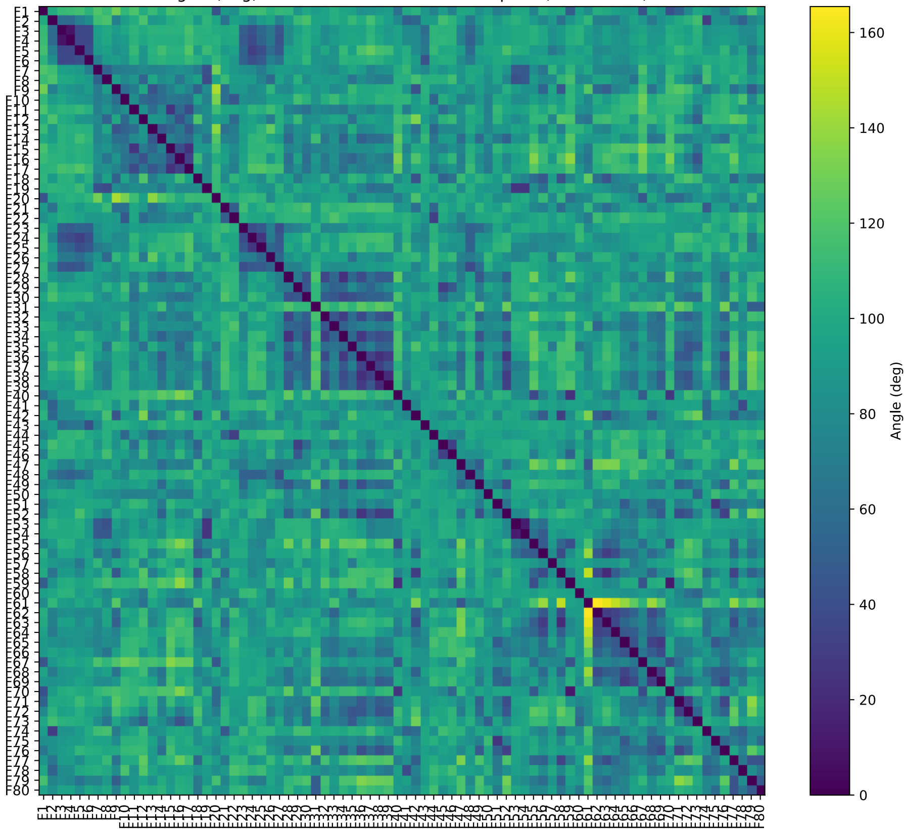
Angles (deg) between feature axes in PC-space (first 12 PCs)
