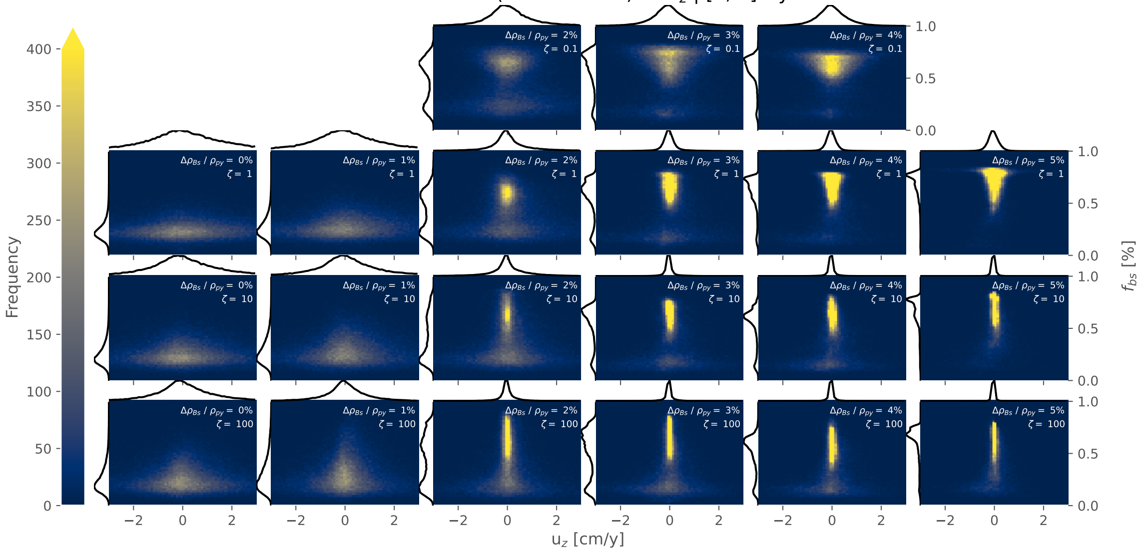
Bs fraction ( z > 2500 km) vs u_z | [4, 5] Gy
