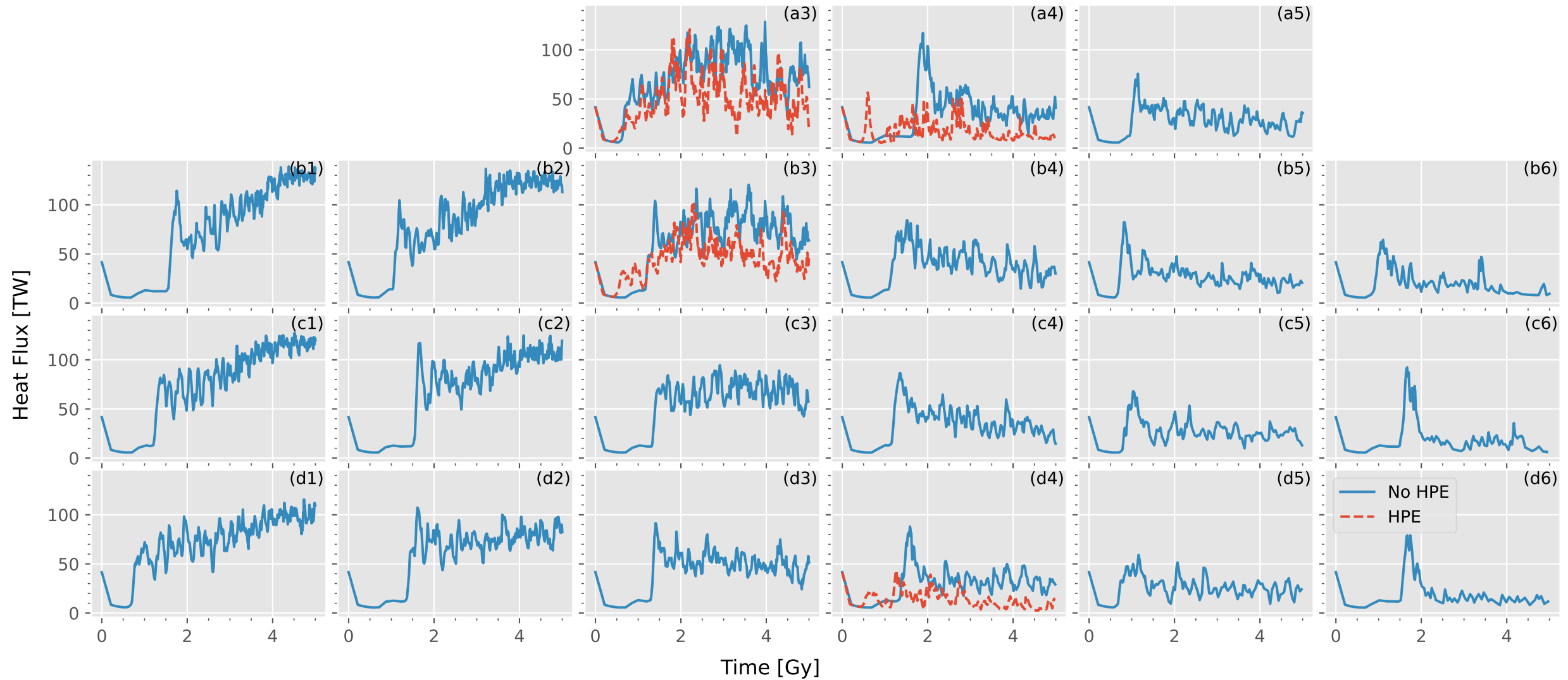
CMB Heat Flux Evolution
