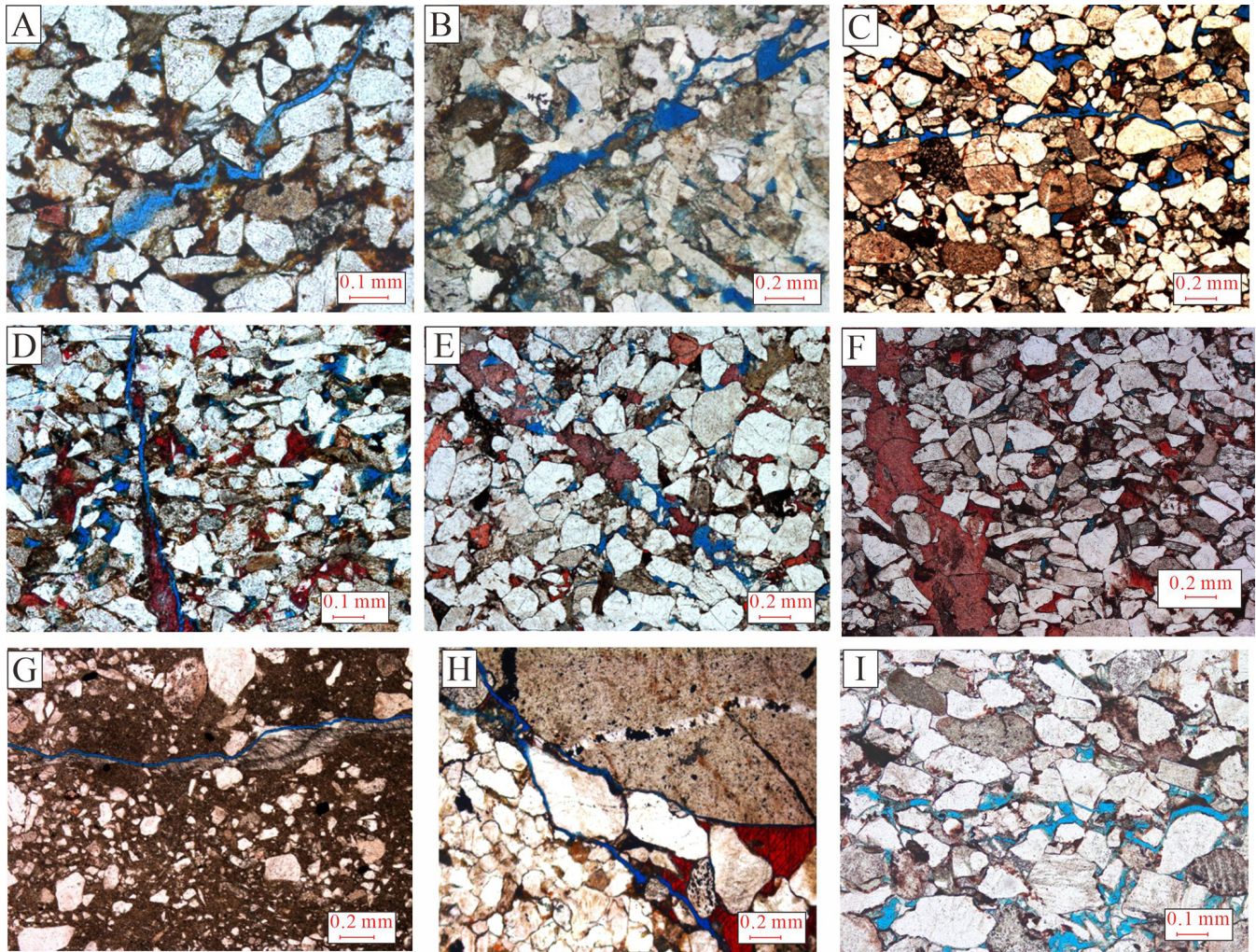
Figure 3. The thin section images of various types of thin section-scale fractures in Bashijiqi Formation in Bozi-Dabei Block of Kuqa Depression (modified from Su et al., 2024). Proposed added reference: Su et al. (2024).
