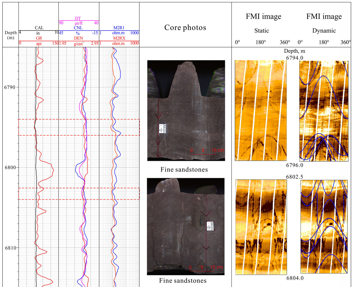
Figure 5. Fracture characteristics in fine-grained sandstones in Well BZ 104 (6785–6815 m). Core photographs showing fracture density characteristics. Fine-grained sandstone interval (6794–6796 m) exhibits higher fracture density.
