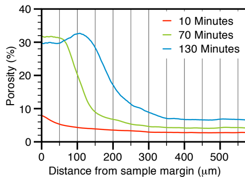
Fig. 4. Distribution of porosity along a radius at 10, 70 and 130 min. Note the slightly increasing background porosity in the inner domain. Values exceeding 30 % porosity result from the comparatively small sampling volume used to determine the porosity values shown.
