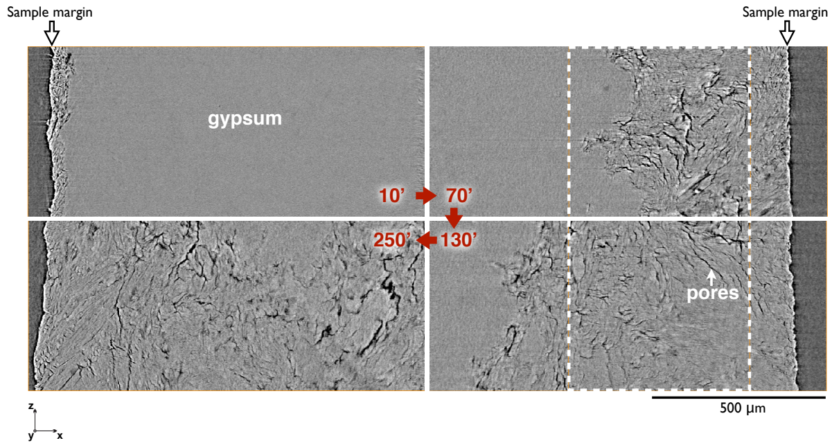
Fig. 2. Vertical cross section through the sample at different times during the experiment (depicted in the four quadrants). The grey values correspond to the absorption of x-rays, pores appear dark grey to black. The white stippled frame outlines the location of the parallelepiped in which porosity was quantified (see text and also Supplement, Fig. 5).
