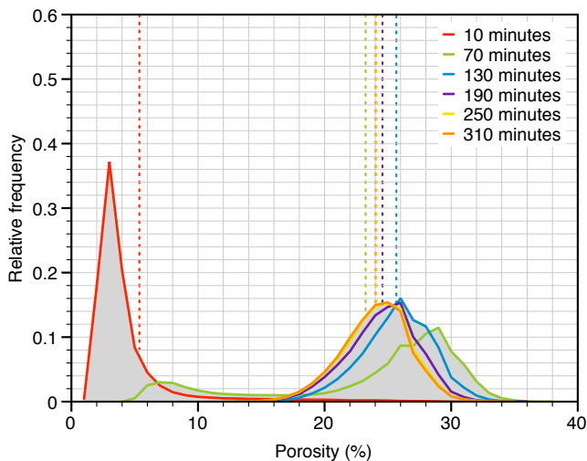
Fig. 12. Porosity frequency distribution amongst cubes with a 50-voxel side length sampled throughout the parallelepiped at different times during the experiment (see text for explanation). The shapes of the peaks give an indication of how homogeneously porosity is distributed within the sample, with the vertical lines marking the total porosity measured at different times. After 130 min the porosity distribution within the parallelepiped is relatively homogeneous.
