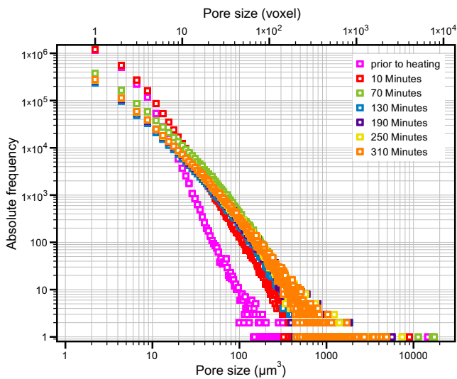
Fig. 7. Absolute pore size frequency distribution over time. The distribution consolidates as soon as the dehydration front has passed through the sampling volume (after 130 min).
