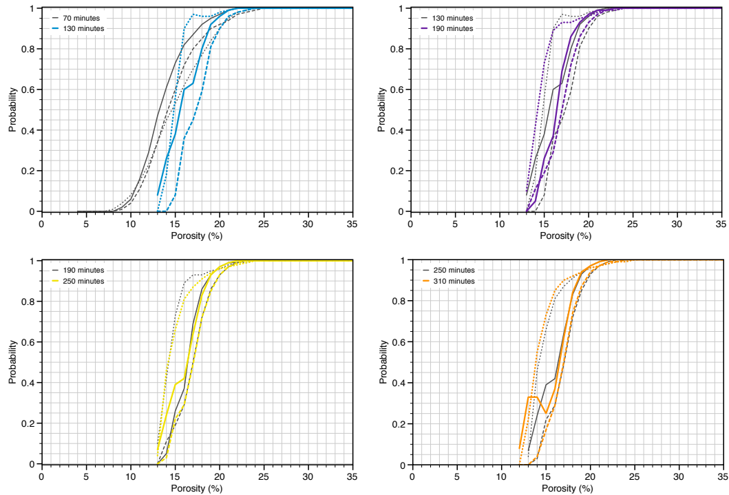
Fig. 13. Probability functions for percolation in the three principal directions amongst cubes with a 50-voxel side length placed in the parallelepiped. Each of the four diagrams compares two consecutive time steps. Dotted lines – x-axis, stippled line, y-axis, solid line – z-axis. Note that from 130 min onward, all cubes with more than about 22 % porosity are percolating in all three directions. In all cubes with a smaller porosity, the x-direction is most likely to percolate.
