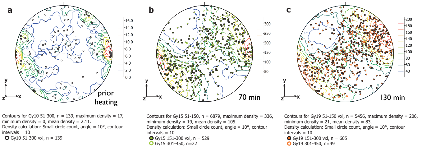
Fig. 11. Stereo plots showing the orientations of the longest principal axis of pores of different sizes. (a) Orientations prior to heating, contours calculated from pores between 51 and 300 voxel, circles denote pores between 51 and 300 voxel in volume; (b) Orientations after 70 min, contours are calculated from pores between 51 and 150 voxel, black circles are orientations of pores between 151 and 300 voxel and green circles of pores between 301–450 voxel; and (c) Orientations after 310 min, contours are calculated from pores between 51 and 150 voxel, black circles are orientations of pores between 151 and 300 voxel and orange circles of pores between 301–450 voxel. The plots indicate that a pre-existing anisotropy controls the orientation of pores before and during dehydration.
