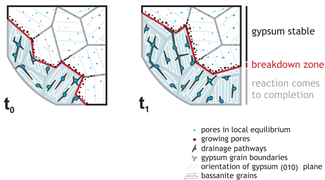
Fig. 14. Sketch map illustrating the grain-by-grain advance of the dehydration front and the effect of the strong crystallographic anisotropy of gypsum. See text for discussion.
