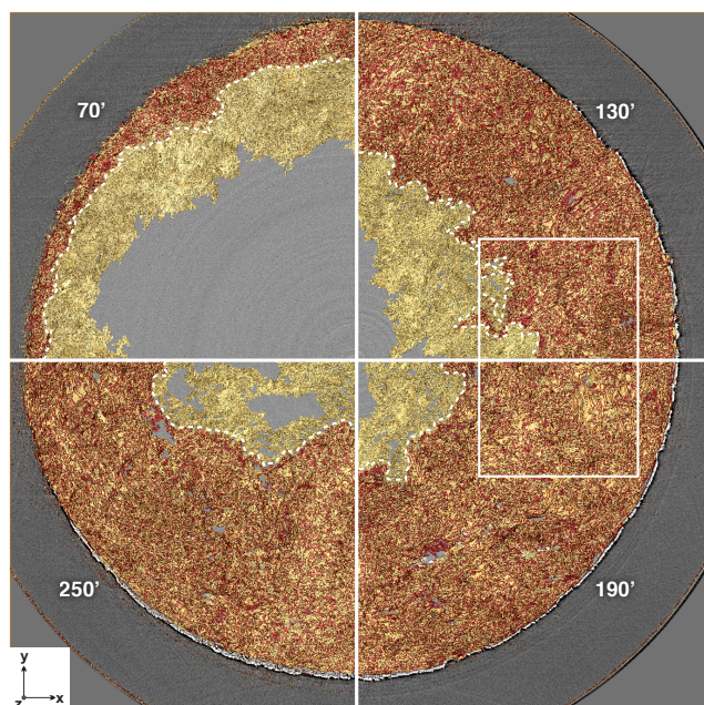
Fig. 9. Horizontal section through the sample cylinder illustrating the largest interconnected pore cluster (in yellow) at different times during the experiment. Each quadrant shows the extent of the cluster at the time indicated, the stippled line indicates the extent of the cluster 60 minutes earlier (in red). The sample diameter is 2.3 mm. The white frame indicates the location of the parallelepiped in which porosity was quantified.
