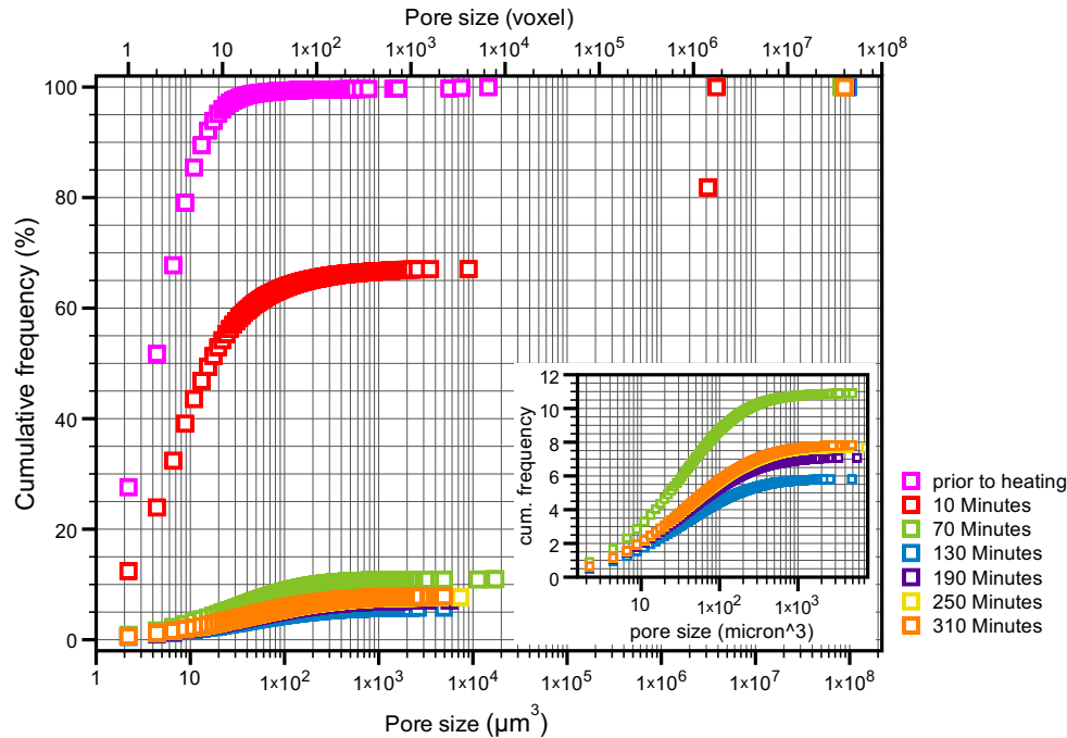
Fig. 8. Cumulative porosity size frequency distribution over time. The distribution is dominated by a single cluster of interconnected pores that makes up more than 90 per cent of the total porosity.
