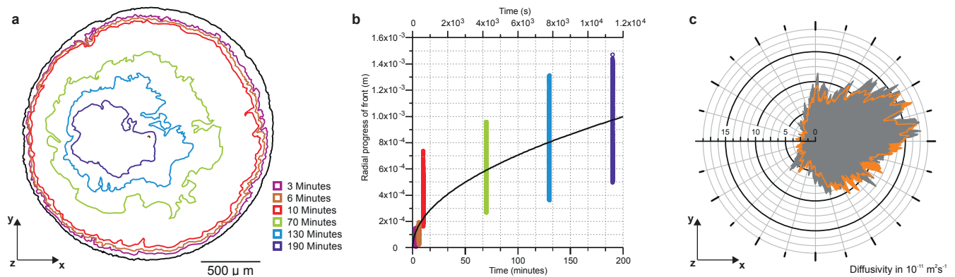
Fig. 5. The advance of the dehydration front, (a) the position of the dehydration front in a horizontal section through the sample at different times during the experiment; (b) the slow, highly non-linear radial progress of the front over time quantified from horizontal and vertical sections through the sample. See text for explanation of the technique. (c) rose plot of linear diffusion constants derived from fitting Eq. 1 to propagation of dehydration front along radii in two horizontal cross sections through the sample. The higher diffusion coefficients probably relate to a pre-existing alignment of gypsum in part of the sample, as discussed in the text. Measurement strategy is explained in text (see also Supplement, Fig. 3).
