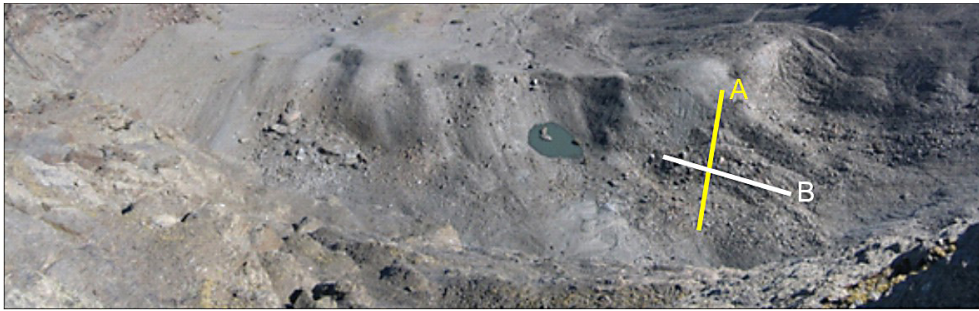
Figure 2. Distribution of the geophysical prospecting transects conducted across the rock glacier in the eastern third of the Corral del Veleta.
