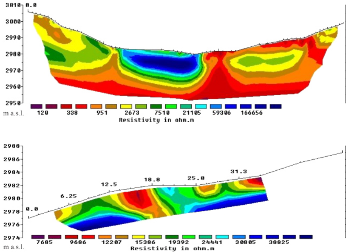
Figure 6. Geophysical prospecting over the whole of transect A, transversal to the rock glacier in its middle stretch and adjacent margins (N–S; top) and transect B, longitudinal to the rock glacier (W–E; bottom) (source: Galindo-Zaldívar).
