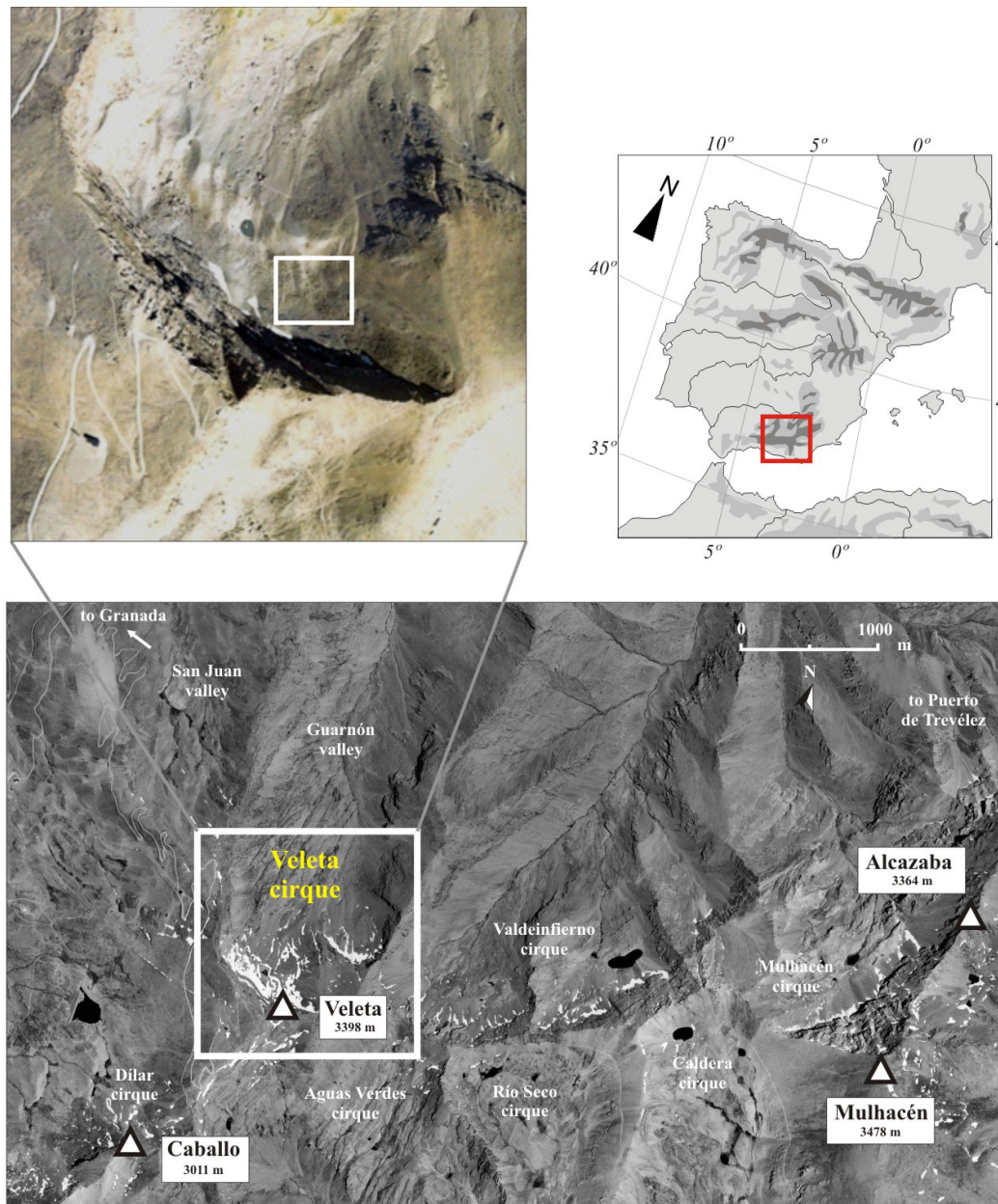
Figure 1. Sierra Nevada peaks and location of the Corral del Veleta.
