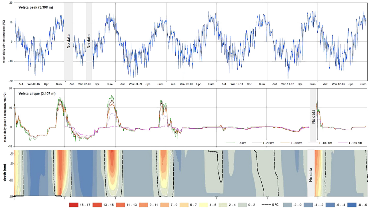
Figure 5. Annual rhythm of ground temperatures at the heart of the rock glacier for 2006–2013.
