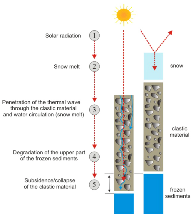
Figure 8. Interpretative diagram of the knock-on physical processes.
