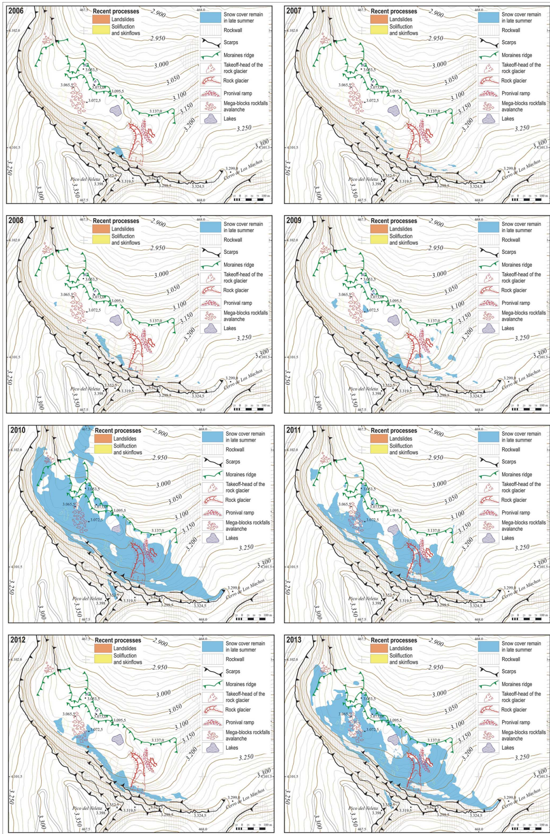
Figure 4. Ground snow cover on the Corral del Veleta at the end of August during the 2007–2011 period.
