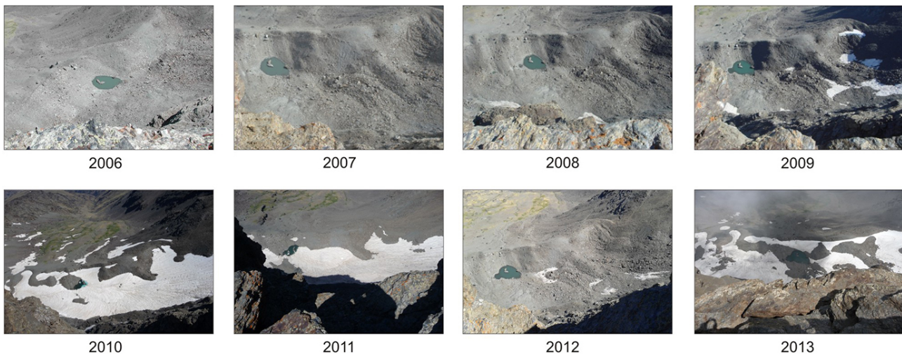
Figure 3. Vertical photographs of snow cover on the Corral del Veleta at the end of August from 2006 to 2013.
