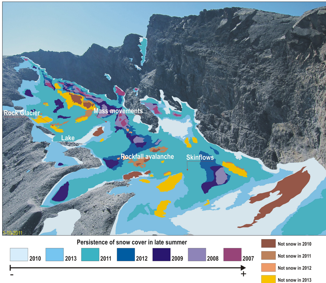
Figure 7. Evolution of snow cover on the Corral del Veleta for 2007–2011.
