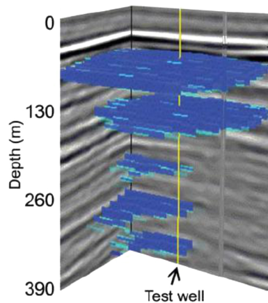
Figure 1. Geometry of a gas reservoir (in blue) deduced from electro-seismics (from Thompson et al., 2007).
