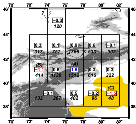
Figure 4. Residuals of the differential time between the P660s and P410s phases in seconds relative to the IASP91. Strongly anomalous boxes (A, B, C) are in south-central Tien Shan (1.5 s, blue), Fergana Basin (−1.1 s, red), and Tarim (−1.5 s, red). Light shading indicates elevations greater than 1500 m, and intermediate shading elevations greater than 3000 m. The number of stacked receiver functions in each box is shown by italics. Permian basalts in Tarim are orange.
