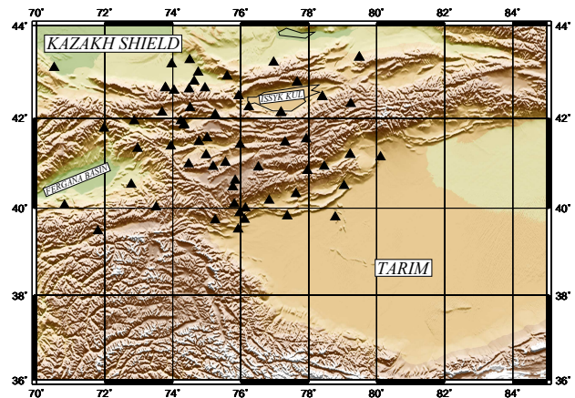
Figure 1. Topographic map of the study region and the seismograph network.
