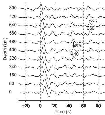
Figure 3. Stacked PRFs for the box with the corners at 38–40° N and 80–82° E. Move-out corrections for stacking are calculated for depth (in km) attached to the traces on the left-hand side. The detected P410s and P660s phases are marked by arrows. Note that the largest amplitudes of the P410s and P660s phases are observed at appropriate trial depths (around 400–500 and 600–700 km, respectively).
