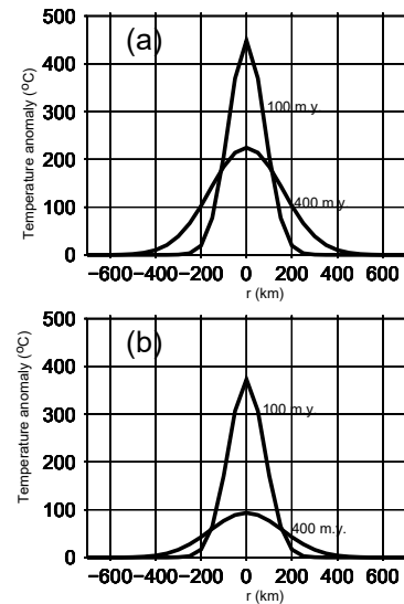
Figure 5. Temperature anomaly distributions in 1-D (a) and 2-D (b) conductive media with an interval of 300 million years.
