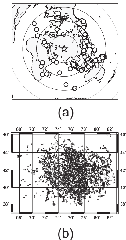
Figure 2. Epicenters of seismic events (a) and projections of piercing points at a depth of 535 km (b).
