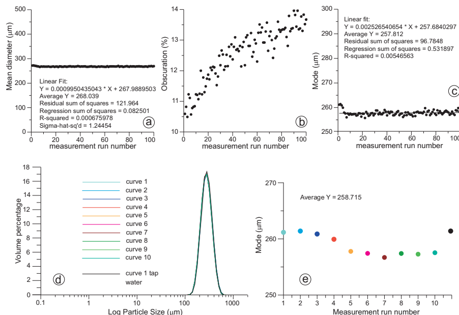
Fig. 17. Results of the chemical test MP2500 5aI performed on sub-sample aliquot SAND1e by the Hydro 2000 MU dispersion unit, using denaturated ethylic alcohol as dispersant liquid. (a) Mean diameter value evolution with increasing the number of measurement runs. Data statistics is provided. (b) Laser obscuration value progression during the same test. (c) Progression of modal values with increasing the number of measurement runs. Data statistics is provided. (d) Granulometric curves computed for the first 10 runs, compared with the first curve from the test MP2500 5 on sub-sample aliquot SAND1c (Fig. 7). (e) Modal values corresponding to the curves in (d).
