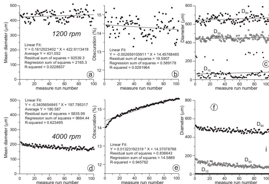
Fig. 9. Comparison between measure precision test results performed on sample CABRE3 at the pump speed corresponding to the mean diameter peak value of the pump speed test (Fig. 3a), and at the maximum pump speed, respectively. (a) Test MP1200 5 performed on sub-sample aliquot CABRE3e by the Hydro 2000 MU dispersion unit; mean diameter value evolution with increasing the number of measurement runs. Data statistics is provided. (b) Laser obscuration value progression during the same test. Data statistics is provided. (c) Progression of D 10 , D 50 , and D 90 percentiles during the same test. (d) Test MP4000 5 performed on sub-sample aliquot CABRE3f by the Hydro 2000 MU dispersion unit; mean diameter value evolution with increasing the number of measurement runs. Data statistics is provided. (e) Laser obscuration value progression during the same test. Data statistics is provided. (f) Progression of D 10 , D 50 , and D 90 percentiles during the same test. Note the very large difference between the average mean diameter obtained from the first (431.052 μm) and the second test (180.587 μm), respectively. Both them are affected by strong recirculation-related mechanical bias.
