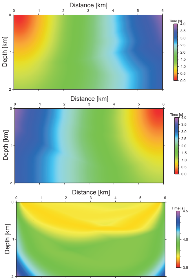
Figure 2. Traveltime tables for the source at x=0.2 km (top) for the receiver at x=5.8 km (middle) and the summation of both timetables (bottom). These traveltime tables were obtained using a finite difference solution of the eikonal equation (Hole and Zelt, 1995). The yellow and orange colors indicate the zone of minimum traveltimes. This illustrates the fastest path from the source to the receiver within the model (the banana-kernels)
