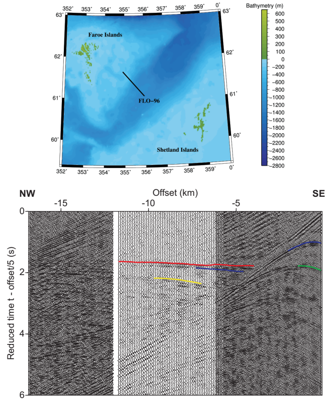
Figure 4. Survey FLO-96. Location map of the profile (top), and shotgather (bottom). In the shot gather the NW corresponds to the left and the SE to the right. The following phases are identified: sea bottom reflection (blue), top-basalt reflection (green), basalt refraction (red), base-basalt reflection (purple) and top-basement reflection (yellow). This shotgather is a composite from the two-ship experiment (see the text for an explanation).
