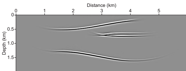
Figure 3. Migrated image of the synthetic example.
