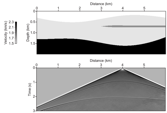
Figure 1. Velocity model used to calculate synthetic data (top) and a shotgather generated at x = 4 km (bottom).
