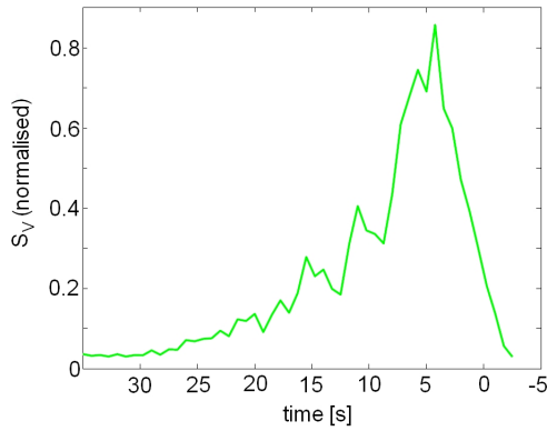
Fig. 13. Time evolution of the normalised S_V = \int_V \epsilon_{xy}^2 d^3 \mathbf{x} for a volume V that extends 20 km by 20 km around the epicentre as estimated from the time-reversal images from figure 12. The peak occurs at +3 s relative to the focal time estimated by Semmane (2005) ( t = 0 ).
