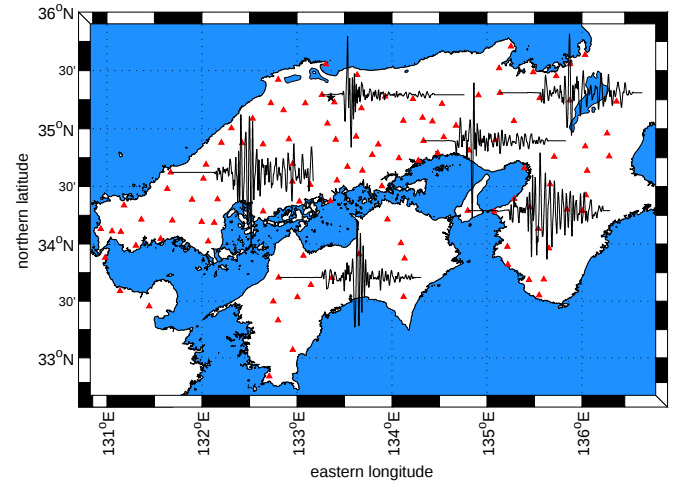
Fig. 11. Source-receiver geometry of the real-data TR experiment for the 2000 Tottori earthquake. Red triangles mark the positions of the 111 stations used in the experiment, and the black star indicates the epicentre as inferred by Semmane (2005). The seismograms shown are vertical component velocities in the chosen frequency band.
