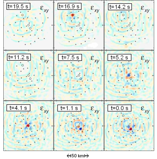
Fig. 4. Snapshots of the time-reversed strain field \epsilon_{xy} at 12.5 km depth. Receiver and source locations are indicated by + and o, respectively. Focusing at all three source locations can be observed with an uncertainty of \sim 5 km in space and \sim 1 s in time. The observed hypothetical rupture velocity is 2 \pm 0.3 km/s, compared to 2 km/s used to generate the forward wave field.
