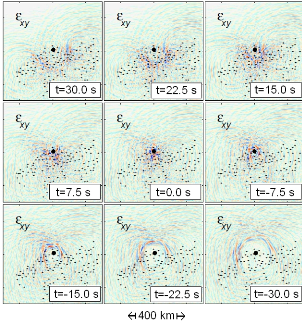
Fig. 12. Snapshots of the time-reversed strain component \epsilon_{xy} at the surface for the Tottori data recorded at the 111 stations shown in figure 11. The coastlines are omitted to enhance the visibility of the time-reversed field. Estimates of both the focal time ( t = 0 s) and the epicentre location (black dot) are taken from Semmane (2005).
