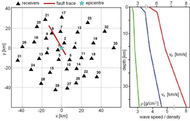
Fig. 1. Left: Geographic model setup. Stations are marked by triangles. The red line and the star mark the fault trace and the epicentre for the finite-fault simulations in section 4. Right: Velocity and density model used in all synthetic simulations.
