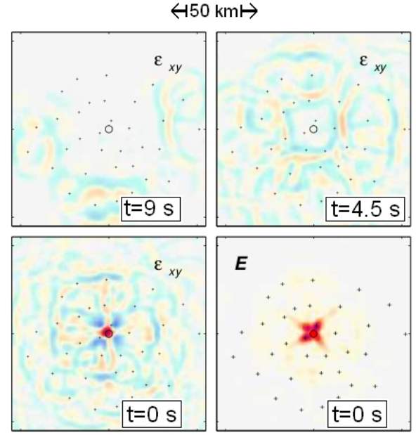
Fig. 3. Snapshots at the point-source depth (12.5 km) of the time-reversed strain field \epsilon_{xy} at different times, and the energy \frac{1}{2}v^2 (lower right) at t=0 .
