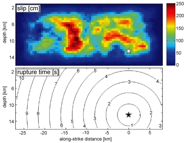
Fig. 6. Synthetic slip (top) and rupture time (bottom) distributions of the SPICE Tottori benchmark (Mai et al., 2007). Both the rupture speed and the rise time are constant at v_r = 2.7 km/s and 0.8 s, respectively
