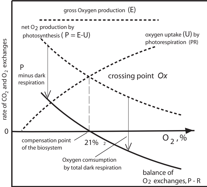
Diagram of gas exchanges of a terrestrial biosystem based on C3 plants
