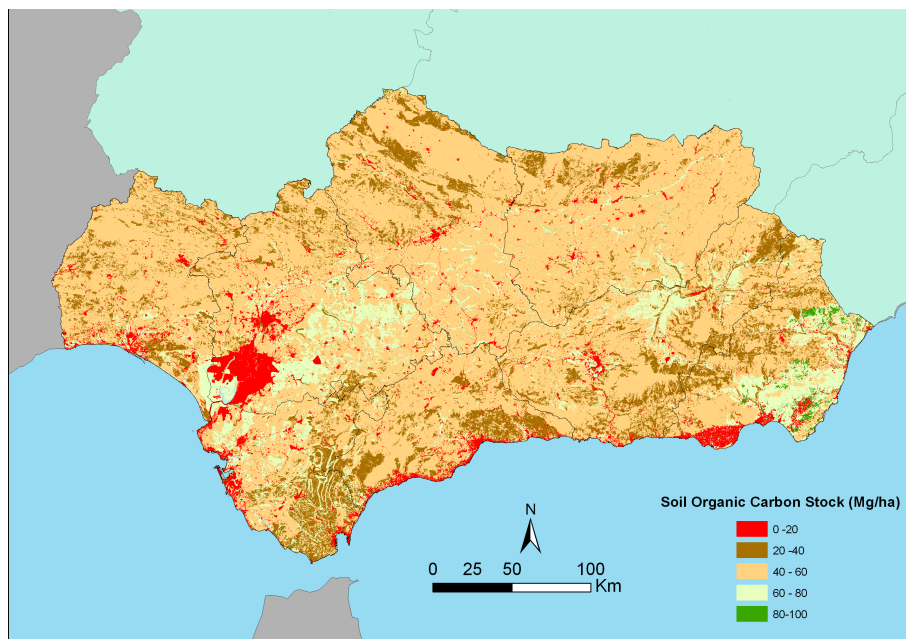
Fig. 6. Map of soil organic carbon content (0–75 cm) in Andalusia.
