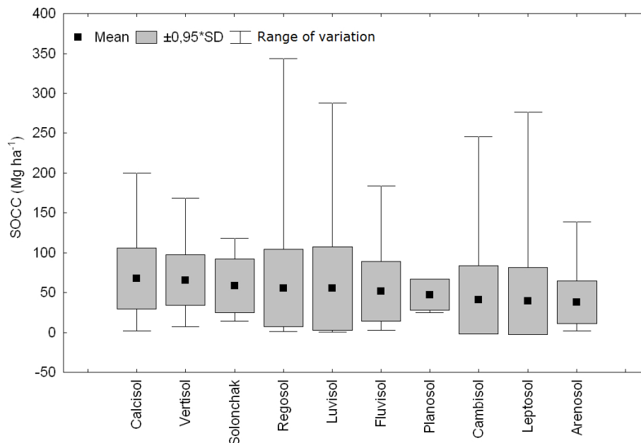
Fig. 2. Soil organic carbon content (SOCC) for the major soil types in the study area. SD: standard deviation.
