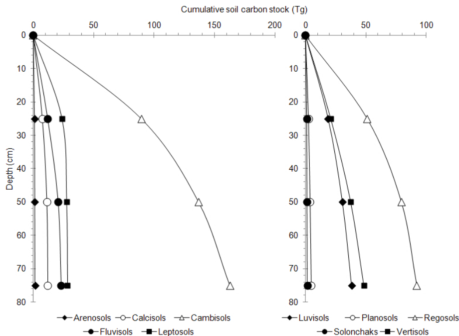
Fig. 4. Cumulative soil organic carbon stock in depth for each soil class.
