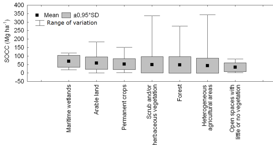
Fig. 3. Soil organic carbon content (SOCC) for each land use type. SD: standard deviation.
