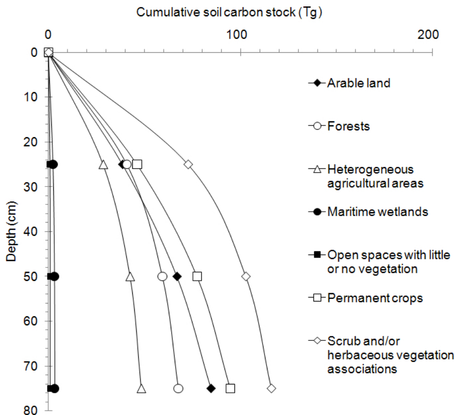
Fig. 5. Cumulative soil organic carbon stock in depth for each land use type.
