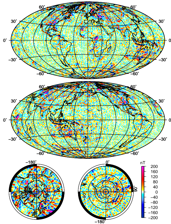
Fig. 8. Map of the vertical down components of the final lithospheric field model B_i . The map has been calculated at the Earth's surface (6371.2 km). Although some noise is still visible in the northern Atlantic and over the southern polar cap, the noise level over mid latitudes has been greatly reduced. Anomalies are particularly well defined over continents, and Indian and Pacific oceans.
