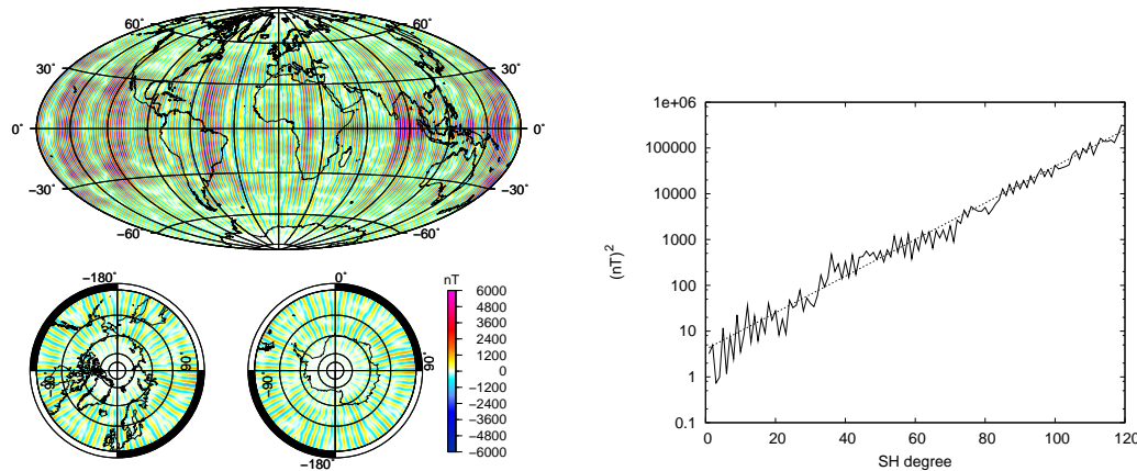
Fig. 2. Left: mapping at r' = 6371.2 km of the model defined in Eq. (13) where l_1^1 = 1 , r = 6671.2 km – i.e. 300 km altitude, and the random variables \chi_m^1 have a variance defined in table 1 using v^l = M . Right: associated power spectrum. The dashed line is proportional to (\frac{r}{r'})^{2l} .
