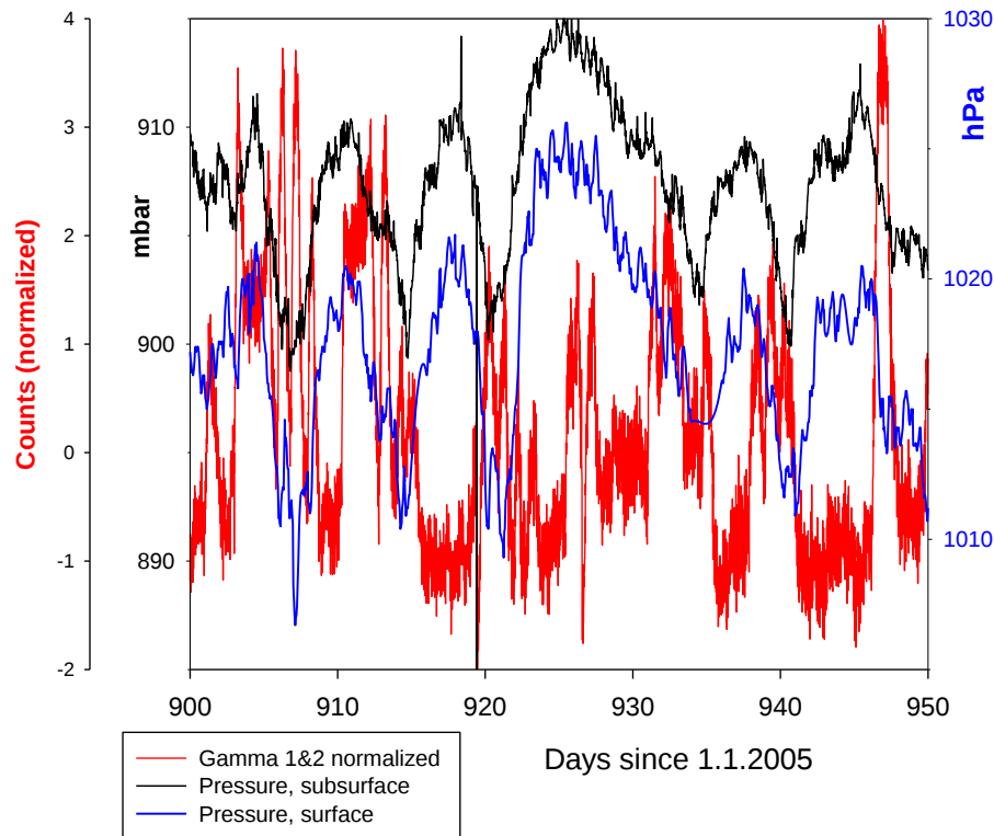
Fig. 8. Time series (50 days) of air pressure both in the subsurface lab and at surface along with concurrent variation of the gamma radiation due to radon in the air of the room. All time series are dominated by multiday signals. The subsurface pressure varies according to the above surface pressure. The variation of radon shows a different pattern.
