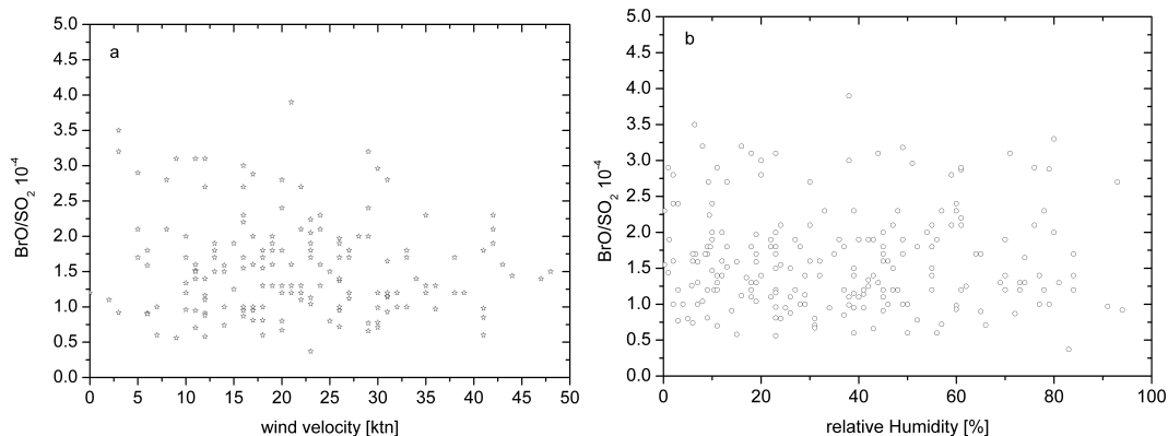
Fig. 5. (a) BrO/SO 2 ratio taken in a distance of about 6 km from the summit of Etna shown as a function of wind velocity, data taken from ( http://weather.uwyo.edu/upperair/sounding.html ) for the day of measurements and altitude of about 3000 m, no dependency visible. (b) BrO/SO 2 ratio taken in a distance of about 6 km from the summit of Etna shown as a function of relative humidity, data taken from ( http://weather.uwyo.edu/upperair/sounding.html ) for the day of measurements and altitude of about 3000 m, no dependency visible.
