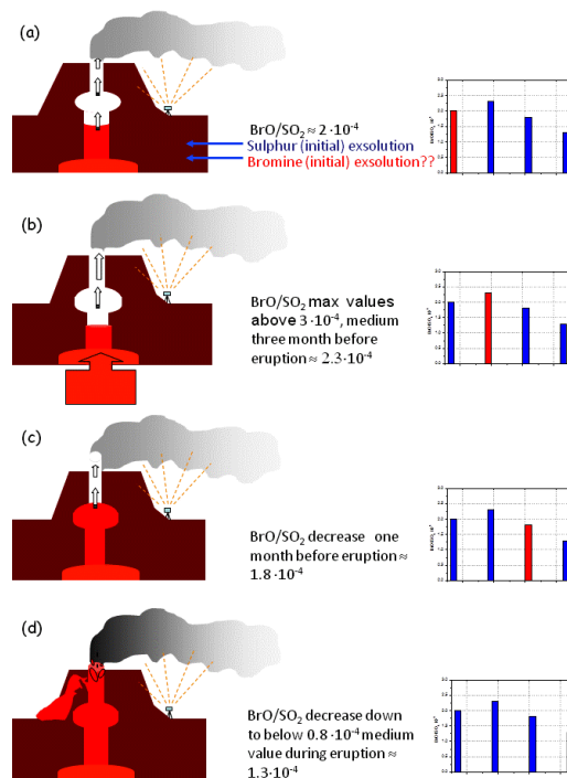
Fig. 7. Sketch of the empirical model, for detailed information see text. (a) In contrast to chlorine and fluorine, we assume that bromine is less soluble in the magmatic melt than sulphur. The mean value of non-eruptive periods during 2006–2009 is around 2 \times 10^{-4} . (b) Assuming bromine is less soluble in magmatic melt than sulphur, bromine starts to be released earlier in comparison to sulphur when fresh magma is rising up –> maxima \text{BrO/SO}_2 ratios rise over 3 \times 10^{-4} . The mean value is around 2.3 \times 10^{-4} in month three before the 2006 and 2008 eruptions as well as in month three and two before the two violent lava fountaining events in 2007. (c) When magma is rising further, sulphur starts to be released and might overtake bromine; \text{BrO/SO}_2 ratios decrease ( \text{SO}_2 fluxes should increase). The mean \text{BrO/SO}_2 value of the last month before the observed eruption is 1.8 \times 10^{-4} . (d) Further decrease – no further magma rise from below, melt already depleted in bromine, sulphur out-gasing is determining the ratio. The lowest \text{BrO/SO}_2 value during eruptions observed was 0.47 \times 10^{-4} . The mean \text{BrO/SO}_2 ratio was calculated to 1.3 \times 10^{-4} .
