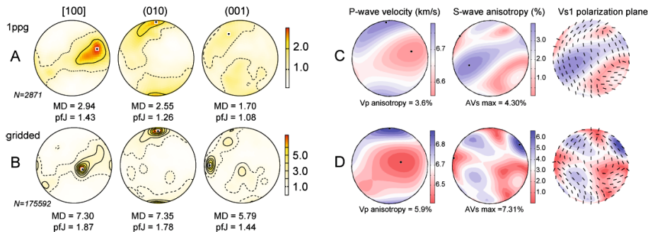
Fig. 8. Seismic properties of sample 176-735B-133R1-35 (ODP Hole 735B oxide gabbro, crystal-plastic microstructure). Plagioclase CPOs plotted from 1 ppg ( a ) and gridded ( b ) data (see Sect. 3.1 for further explanation). Seismic properties are calculated from 1 ppg ( c ) and gridded ( d ) data. The differences between 1 ppg data and gridded data reflect the effect of the heterogeneity of grain size. Contours are multiples of uniform density; V_p is the three-dimensional distribution of the P wave velocity; anisotropy is 100(V_{p_{\max}} - V_{p_{\min}})/(V_{p_{\text{mean}}}) ; AVs is the three-dimensional distribution of the polarization anisotropy of S waves due to S wave splitting; and VS1 is the velocity of the fast S wave (S1); each small segment represents the orientation of the polarization plane at the point at which S1 penetrates the hemisphere.
