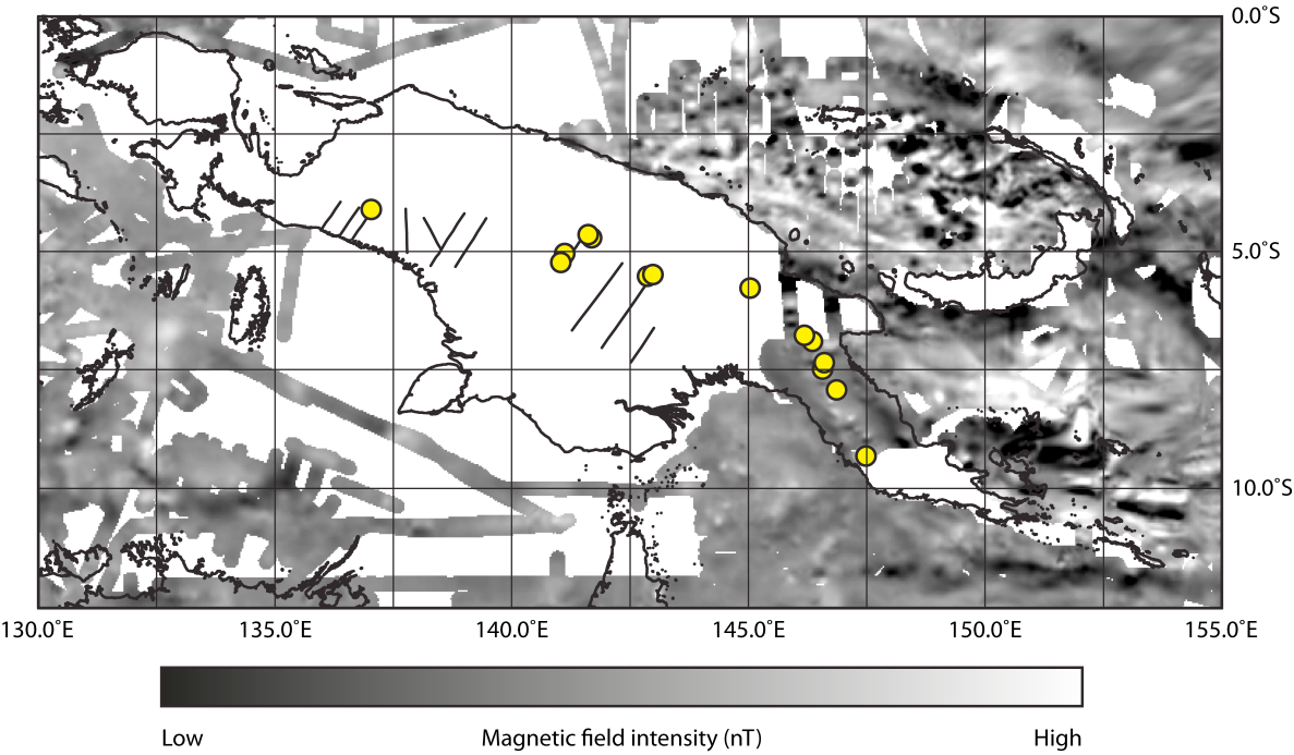
Supplementary File 1: Supplementary File 1: EMAG2 Magnetic Map of N. Australia and New Guinea (Maus et al. 2009)
