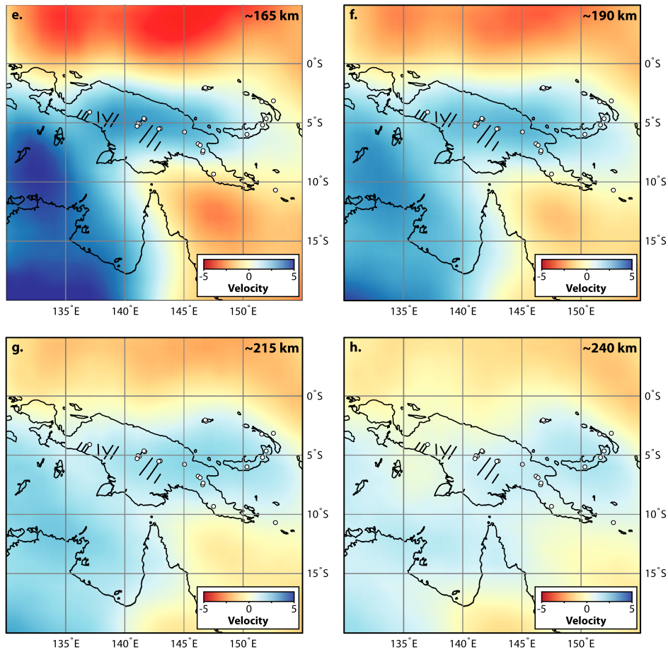
Supplementary Data 2. S-Wave tomography depth slices after the global S-Wave tomography dataset of Debayle et al. (2005). Various slices are shown at (a) ~65 km, (b) ~90 km, (c) ~115 km, (d) ~140 km, (e) ~165 km, (f) ~190 km, (g) ~215 and (h) ~240 km.
