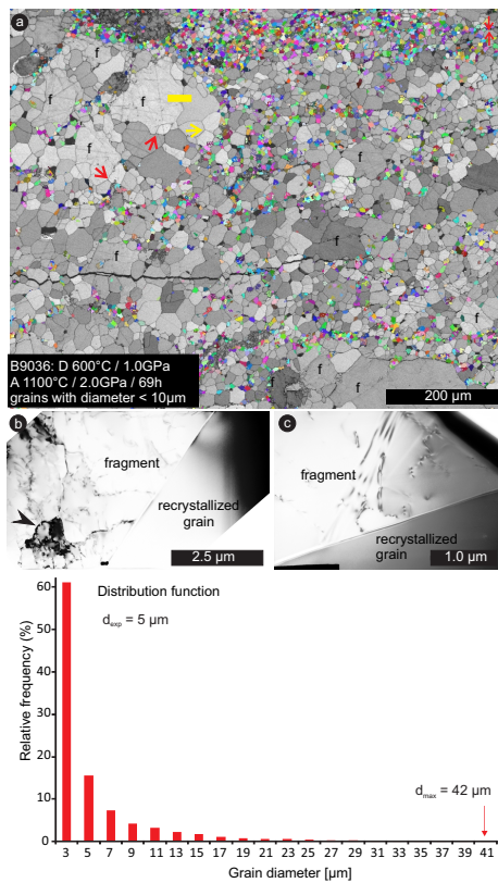
Fig. 2. New Figure 8. EBSD map of sample B9036 with grain size distribution added.
