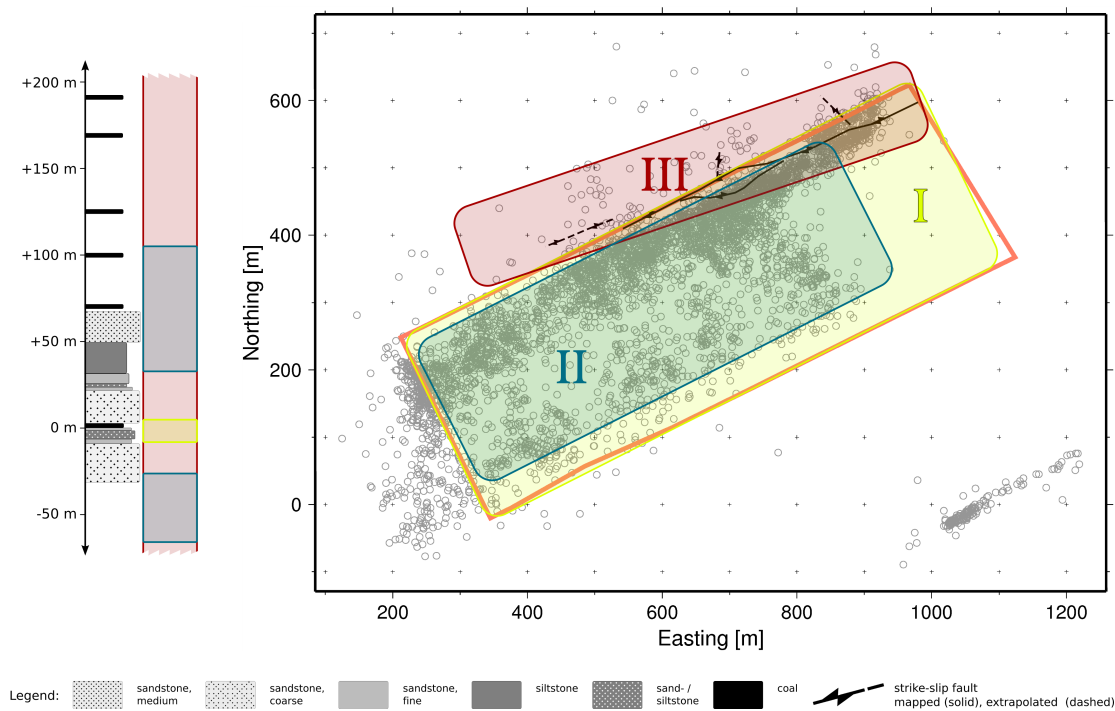
Fig. 1. Mapview of the relocated seismicity of the eight largest clusters (gray circles) and the three main types of brittle failure.
