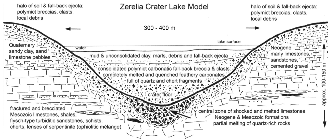
Fig. 12. Magoula Zerelia Crater Lake Model . Approximate dimensions of the larger westerly lake. The basement rocks below the true crater floor are fractured and brecciated but generally show no distinctive shock effects, except in a small zone (outlined by a stippled line) in the center of the structure containing possibly impact melts in form of small lenses. The crater is may be filled, to half its original height, with a variety of breccias. A layer of ejected material (“fall-back breccia”) overlies the uplifted crater rim (halo) and proximal surroundings of the crater.
