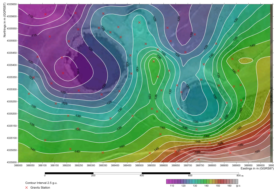
Fig. 8. The reduced Gravity Anomaly Map shows two gravity lows associated with the localities of the two lakes, reaching values of about 115 and 125 gravity units (gu).
