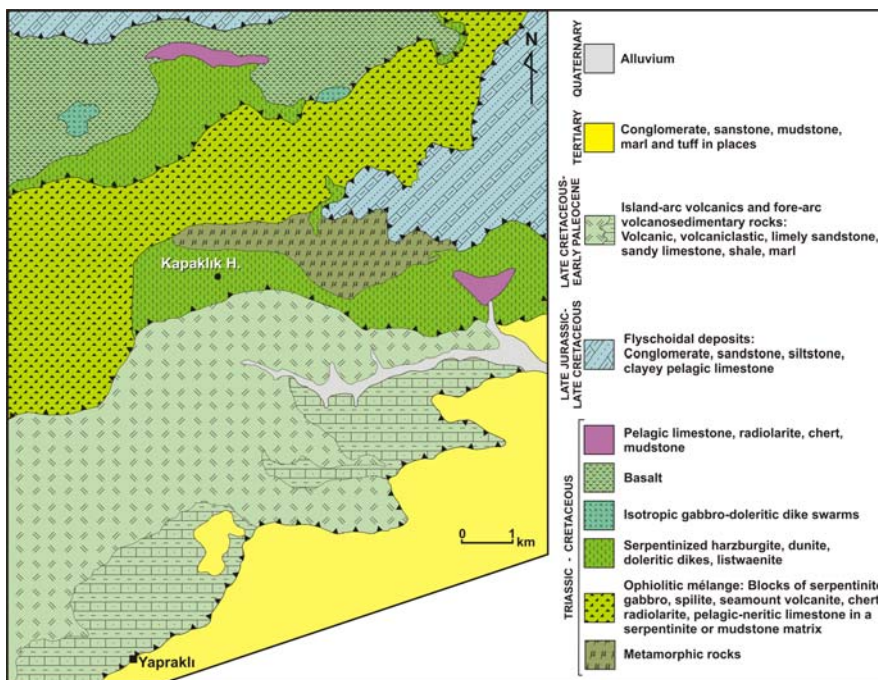
Fig. 6. Simplified geological map of the Yapraklı-Çankırı area, showing the distribution of the ~180 Ma Neotethyan ophiolitic units, ophiolitic mélangé and island-arc rocks.
