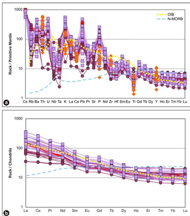
Fig. 17. (a) Primitive mantle-normalized multi-element diagrams for the high-K shoshonitic arc rocks (normalization values from Sun and McDonough, 1989). (b) Chondrite-normalized REE patterns of the same rocks (normalization values from Sun and McDonough, 1989).
