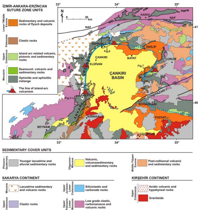
Fig. 2. Geological map of the Çankırı-Çorum area along the IAEZ in north-central Turkey (modified after Uğuz et al., 2002).
