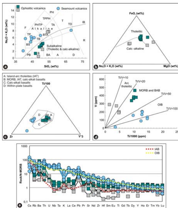
Fig. 13. Geochemical classification of ophiolitic and seamount volcanic rocks. (a) Total alkali vs. \text{SiO}_2 diagram (Le Bas et al., 1986). (b) AFM diagram (Irvine and Baragar, 1971). (c) Ti–Zr–Y discrimination diagram (Pearce and Cann, 1973). (d) Ti–V diagram (Shervais, 1982). (e) N-MORB-normalized multi-element diagrams of the most representative samples (normalization values from Sun and McDonough, 1989). Key to lettering: A = andesite, B = basalt, BA = basaltic andesite, BS = basanite, BTA = basaltic trachyandesite, D = dacite, F = foidite, PC = picrobasalt, PH = phonolite, PHTP = phonotephrite, R = rhyolite, T = trachyte, TA = trachyandesite, TB = trachybasalt, TD = trachydacite, TP = tephrite. IB = alkali-subalkali subdivision from Irvine and Baragar (1971).
