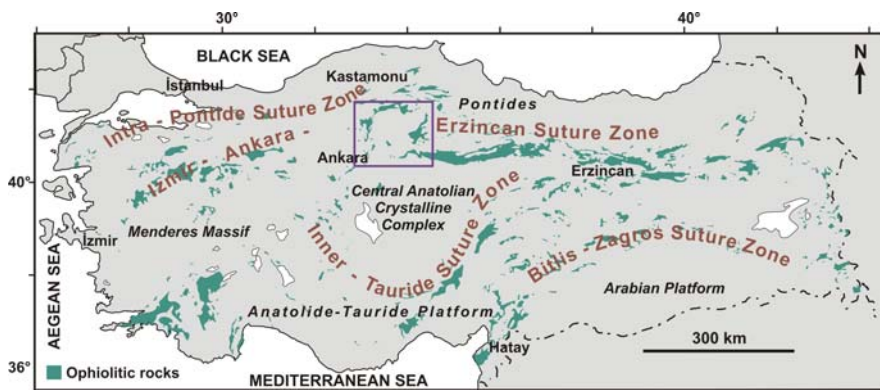
Fig. 1. Simplified ophiolite map of Turkey showing the distribution of the suture zones and some of the major tectonic entities in Turkey (from MTA, 2001). The inset box refers to the map area in Fig. 2.
