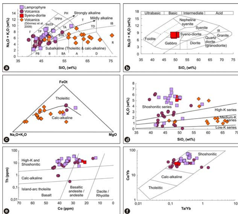
Fig. 14. Geochemical classification of island-arc rocks. (a) Total alkali vs. \text{SiO}_2 diagram (Le Bas et al., 1986). (b) TAS diagram (Cox et al., 1979) for syeno-dioritic pluton rocks. (c) Alk–MgO– \text{FeO}_7 diagram (Irvine and Baragar, 1971) of the subalkaline arc volcanic units (Dönmez et al., 2009, and this study). (d) \text{K}_2\text{O} vs. \text{SiO}_2 diagram (Peccerillo and Taylor, 1976). (e) Th vs. Co diagram (Hastie et al., 2007). (f) Ce/Yb vs. Ta/Yb diagram (Pearce, 1982).
