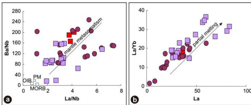
Fig. 18. (a) Ba/Nb vs. La/Nb diagram for the high-K island arc rocks. The data for N-MORB, OIB and PM are from Sun and McDonough (1989). (b) La/Yb vs. La diagram for the island-arc rock units, illustrating the effects of partial melting and fractionation in their melt evolution.
