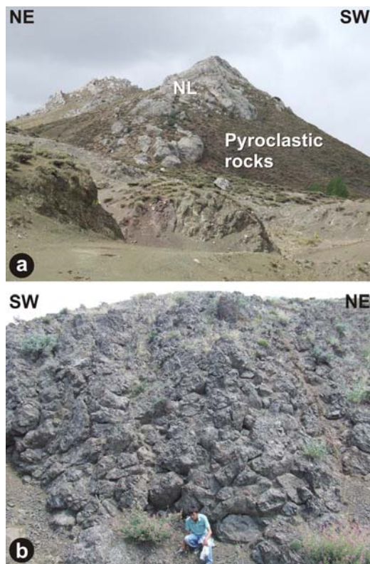
Fig. 8. (a) Neritic limestone covering the seamount volcanic-volcaniclastic rocks in the Ankara Mélange. (b) Seamount pillow lavas in the Ankara Mélange. NL = neritic limestone.
