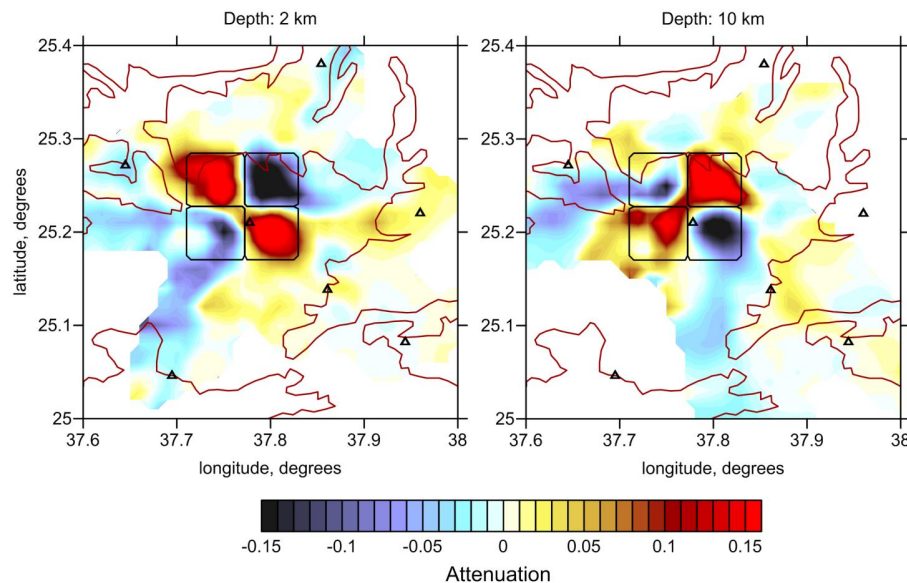
Figure 5. Results of synthetic modeling for the attenuation tomography. Black lines indicate the limits of the synthetic anomalies. At 6 km depth, the anomalies change the sign. Triangles indicate the seismic stations. The contour of the basalt fields is given by brown line for the reference.
