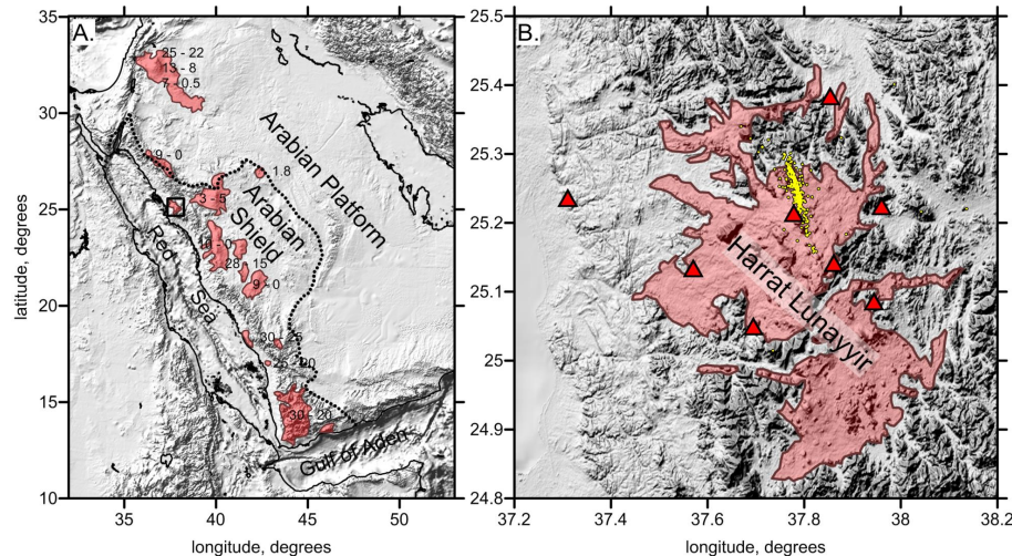
Figure 1. Study region in the framework of regional tectonics and data distribution. (A) Topographic map of the Arabian Peninsula. The dotted line indicates the boundary between the Arabian Shield and the Arabian Platform. The reddish spots mark the Cenozoic basaltic fields (harrats) with their activity ages. The black rectangle is the location of the Harrat Lunayyir. (B) Zoom in of the study area. The triangles show the seismic stations, and the yellow dots mark the event locations used in this study.
