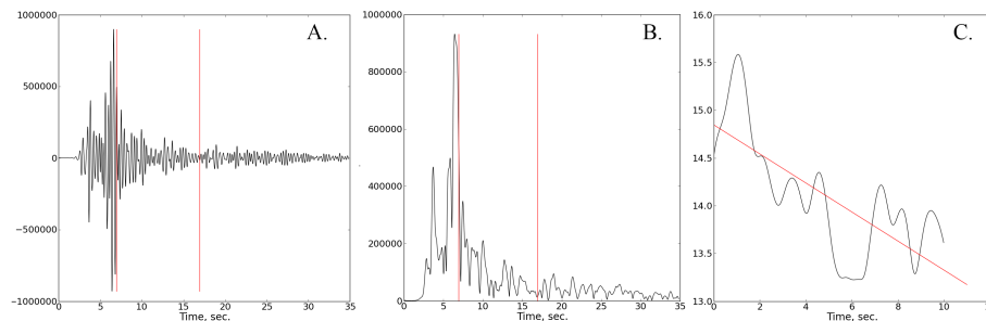
Figure 4. Workflow for the data analysis. (A) Initial seismogram is narrow-band filtered at 3 Hz. The red lines indicate the analyzed time interval. (B) An envelope of absolute deviations in the seismogram. (C) Logarithmic transformation of the envelope. The red line indicates the linear approximation with the best fit. The slope of this line was then converted into the quality factor.
