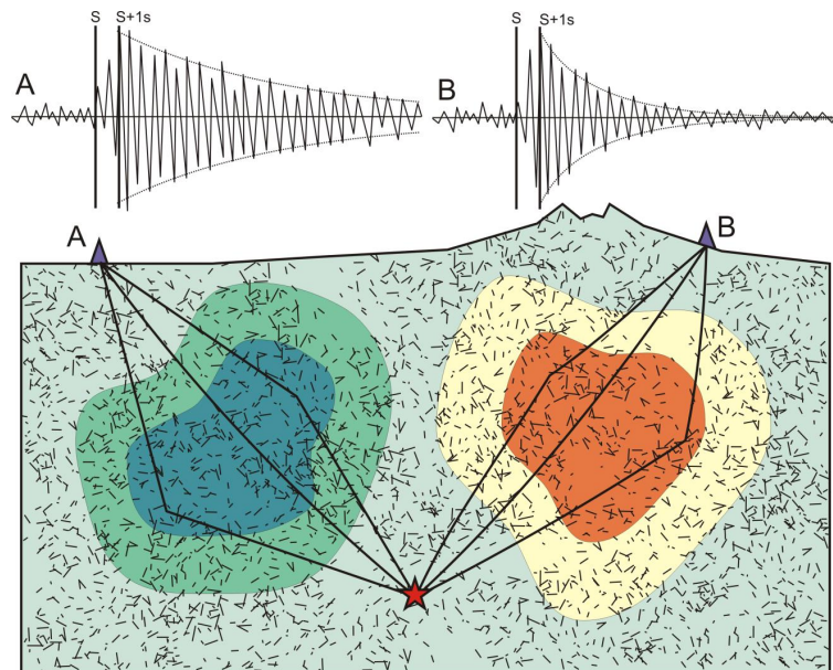
Figure 3. Schematic representation of the basic principle used for the attenuation inversion in this study. Hatches are the scatters which are roughly uniformly distributed within the study area. Red and blue indicate zones of high and low attenuation, respectively. Star is a source; triangles are the receivers; black lines are the direct and scattered rays between source and receivers. Above: schematic seismograms recorded at stations A and B corresponding to low and high attenuation areas. Dotted lines are the envelopes of the seismograms. Lines indicated with S and S + 1\text{ s} mark the arrival time of the S wave and 1 s later point.
