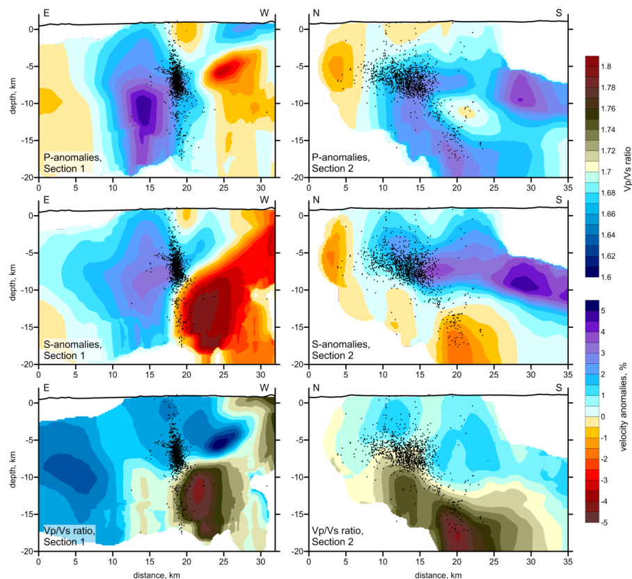
Figure 2. Velocity model ( P , S anomalies and V_p/V_s ratio) and local source hypocenters (black dots) from Koulakov et al. (2014) in two vertical sections with the same locations as shown in Fig. 7. This model and source coordinates were used to construct the rays for the attenuation tomography in this study.
