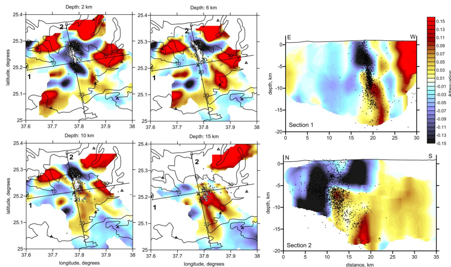
Figure 7. Resulting 3-D distribution of the attenuation in four horizontal and two vertical sections. The dots indicate seismic events near the sections. The triangles are the seismic stations. The black line is the boundary of the basaltic field.
