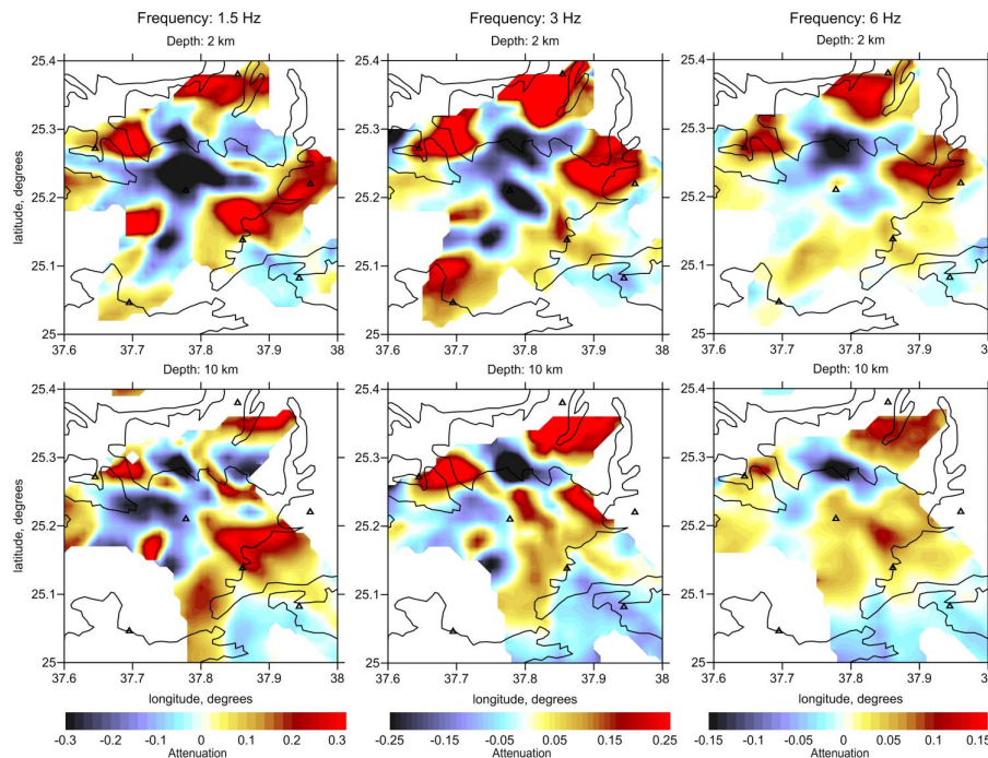
Figure 6. Comparison of the inversion results obtained for the data corresponding to three frequencies: 1.5, 3 and 6 Hz. The results are presented for 2 km and 10 km depth. The triangles are the seismic stations. The black line is the boundary of the basaltic field.
