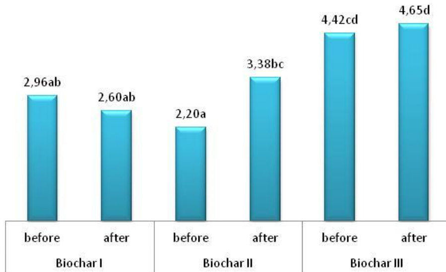
Fig. 1. Evolution of organic carbon oxidised with dichromate.
