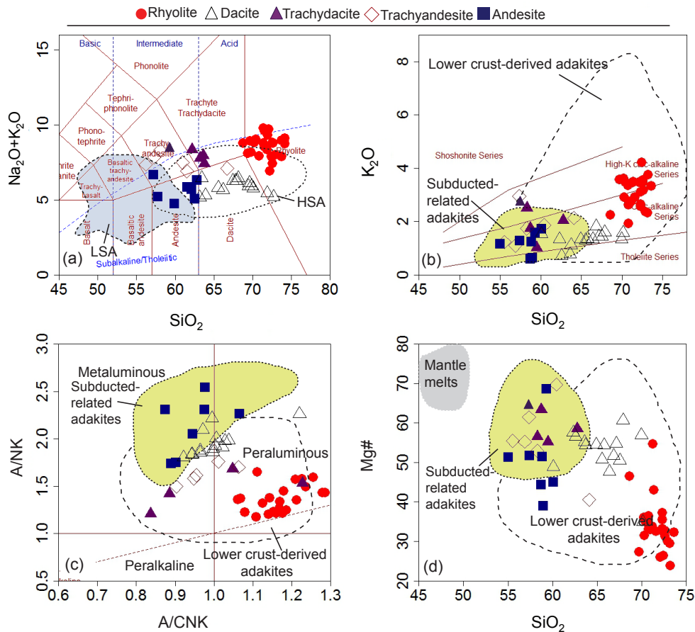
Fig. 1. Fig. 5 Selected major element plots for the subvolcanic post-ophiolite rocks. (a) Total alkalis vs. silica diagram after Le Bas et al. (1986). The boundary between alkaline and subalkaline series is a
