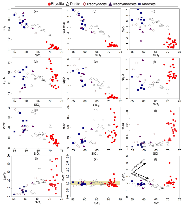
Fig. 2. Fig. 6 Harker diagrams of the major oxides (wt. %) and incompatible element ratios vs. \text{SiO}_2 for the studied rocks.
