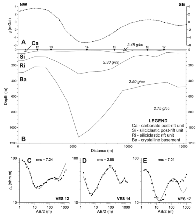
Figure 9. Observed (dots) and calculated (solid line) gravity anomaly across the Profile P02 (A) and the final model response obtained from joint inversion method (B). Comparison of three VES data (dots) and model responses of the gravity–geoelectric joint inversion (C to E). rms: VES misfit (per cent).
