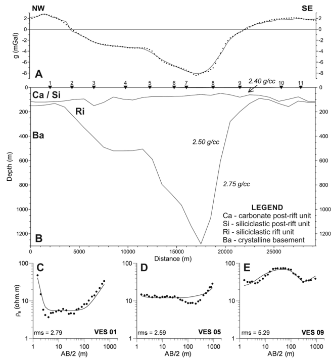
Figure 8. Observed (dots) and calculated (solid line) gravity anomaly across the Profile P01 (A) and the final model response obtained from joint inversion method (B). Comparison of three VES data (dots) and model responses of the gravity–geoelectric joint inversion (C to E). rms: VES misfit (per cent).
