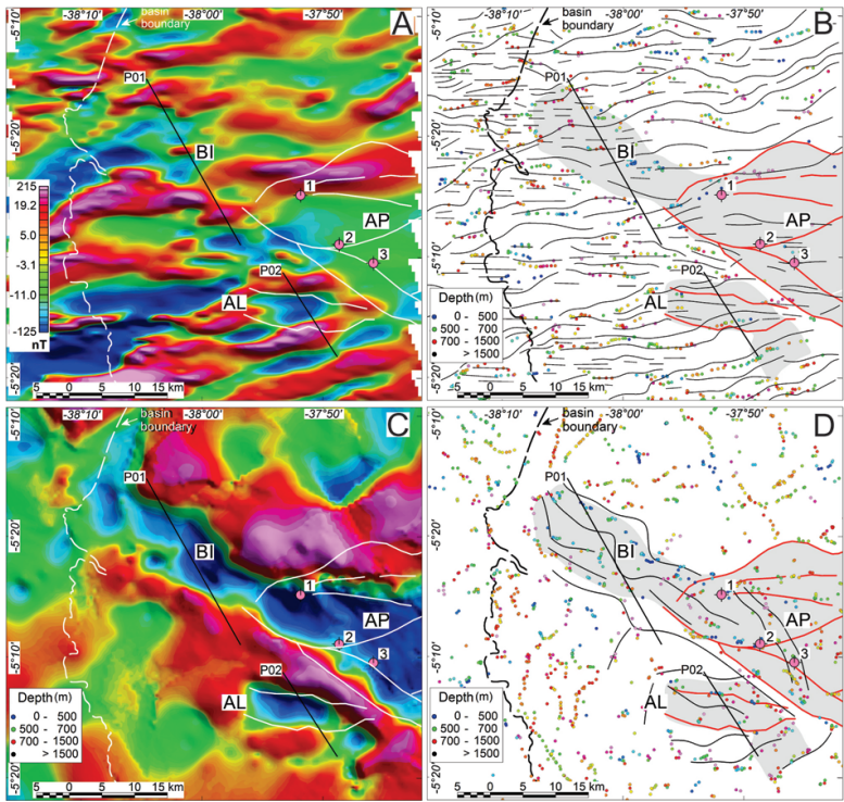
Figure 2907 (A) Residual component of the magnetic field reduced to the pole and (B) major magnetic lineaments and Euler solutions; (C) Residual gravity anomaly map and (D) major gravity lineaments and Euler solutions. (Grabens: (A) – Bica, (B) – Apodi and (C) – Algodões; Profiles: P01 and P02; Exploratory wells: 1, 2 and 3). White and red traces: rift structures from previous studies
