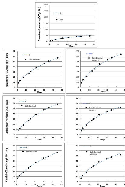
Figure 3. Exponential model of measured C mineralized (as \text{CO}_2 ) and that calculated by addition of soil and BI, BII and BIII effects.
