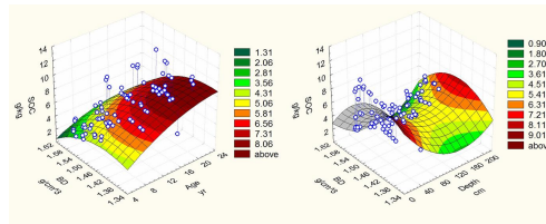
1 2 3 Figure 5. Regression models of soil organic carbon (SOC) and bulk density (BD) with 4 extension of stand age and soil depth.
