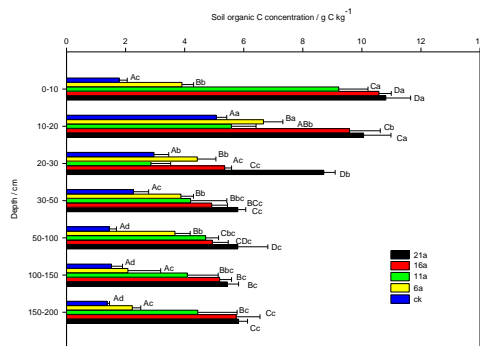
1 2 3 Figure 3. Variations in soil organic carbon concentration at different soil depths in different 4 stand ages. Values are means \pm SE. Different uppercase letters indicate significant differences 5 in different stand ages, different lowercase letters indicate significant differences at different 6 soil depths ( P < 0.05 ).
