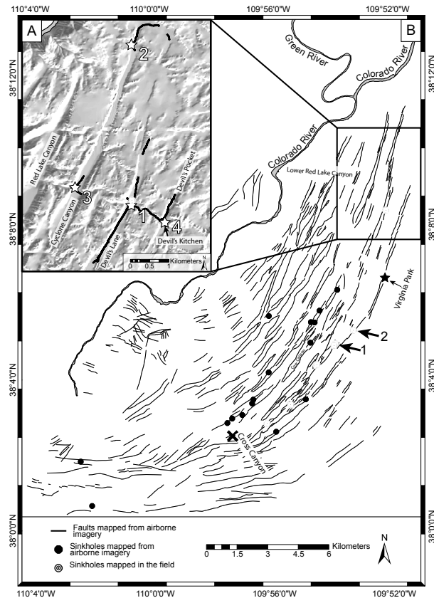
Figure 3. (a) Needles Area, northern part of the Grabens as a hillshade digital elevation model (National Elevation Dataset, NED). Presented GPR profiles indicated by numbered stars. Entire collected GPR dataset is shown by black lines. (b) Overview of the Canyonlands grabens. Graben-bounding faults mapped via orthoimagery. Sinkholes mapped in the field and from imagery.
