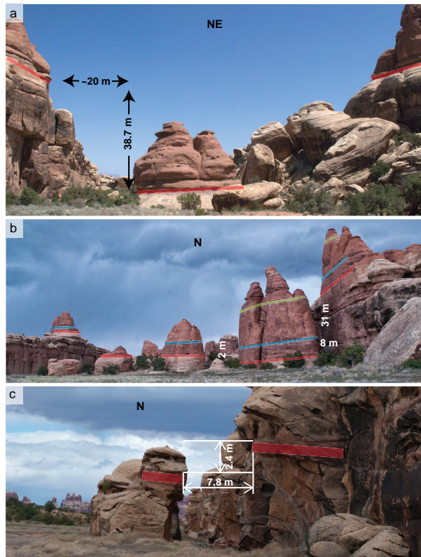
Figure 6. Three locations where heave and throw were measured and fault-dips at depth were estimated. (a) Northern Devil's Pocket. (b) Southern Devil's Pocket. (c) Unnamed graben east of Cow Canyon. Individual heave and throw values are given in images.
