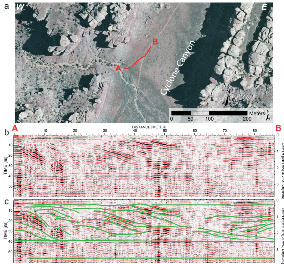
Figure 10. SW–NE profile crossing the central Cyclone Canyon. (a) Aerial photograph illustrating the trace of the profile (red line). (b) 400 MHz Profile without interpretation. (c) Profile with interpretation (green lines: interpreted layers, dashed line: interpreted faults).
