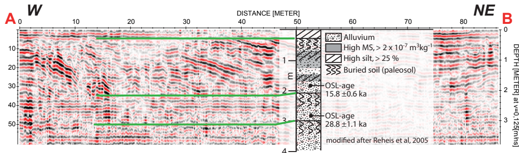
Figure 16. 400 MHz profile of central Cyclone Canyon with overlay of the profile and OSL-ages of Reheis et al. (2005). Three horizontal layers in the GPR profile fit well to paleosols from outcrop profile with an error of less than 0.5 m.
