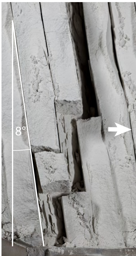
Figure 13. Top view image showing an analogue experiment of Kettermann (2012) with 8^\circ fault-joint angle after deformation. Main fault localized at preexisting joints exclusively; open gaps formed where the shallower dipping fault cuts the vertical joints. Original joint surfaces are preserved.
