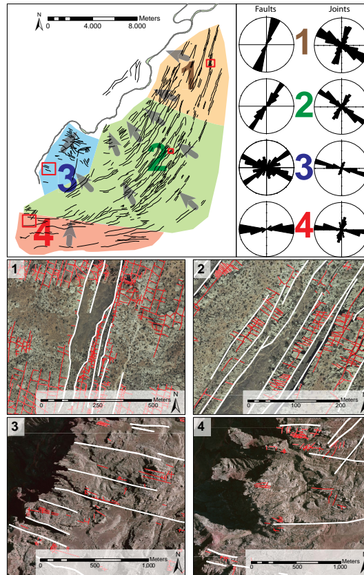
Figure 4. Fault and joint orientations in the Needles Fault Zone derived from airborne image mapping. Four sections group areas of similar orientations. One joint set is always parallel to the major faults. Small red rectangles depict locations of associated detail photographs showing the interpretations of faults (white lines) and joints (red lines). Numbers 1–4 on the photographs correspond to the sections.
