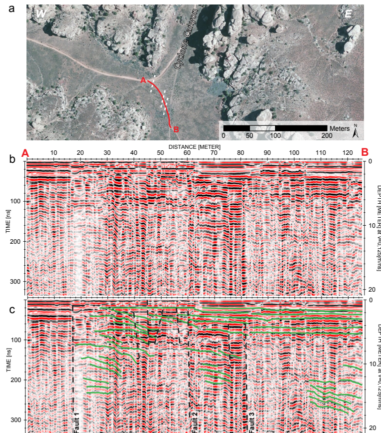
Figure 9. NW–SE profile in northern Cyclone Canyon. (a) Airborne image illustrating pathway of the profile. (b) 100 MHz profile without interpretation. (c) Profile with interpretation (green lines: interpreted layers, dashed line: interpreted faults).
