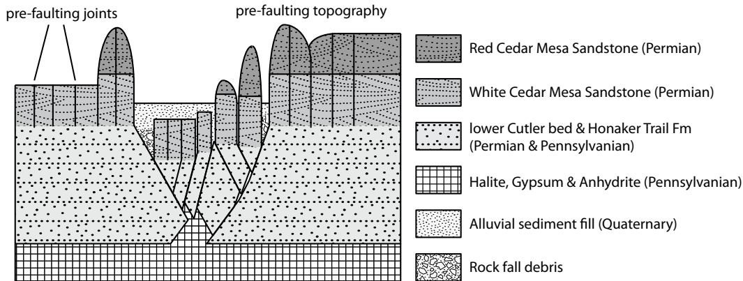
Figure 15. Schematic model of a typical Canyonlands graben from the northern section. Joints of the Cedar Mesa sandstones are reactivated by faulting. Shallower fault dips at depth causes open gaps at surface and secondary faulting within the grabens. Rock fall debris and Quaternary alluvial sediments fill up open gaps and graben floors.
