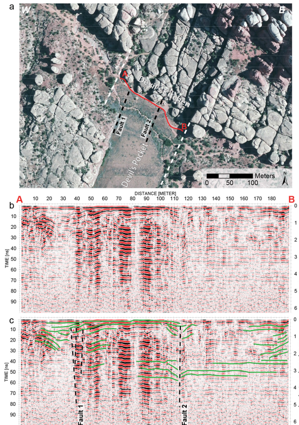
Figure 11. Devil's Kitchen WNW–ESE profile. (a) Aerial photograph showing location of the profile, interpreted faults (black lines) and known graben bounding faults (white lines). (b) 400 MHz profile without interpretation. (c) Profile with interpretation (green lines: interpreted layers, dashed line: interpreted faults).
