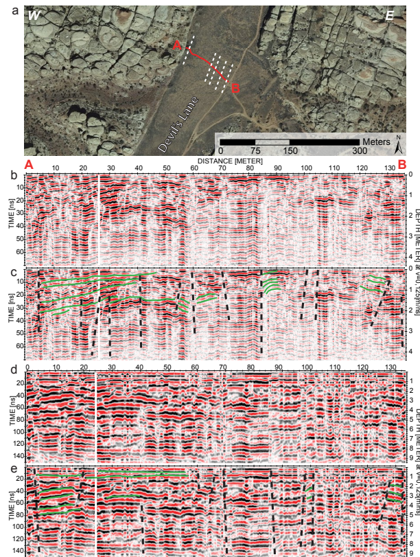
Figure 8. WNW–ESE profiles crossing through Devil's Lane. (a) Aerial photograph of the profile (red line). Interpreted faults are indicated by white dashed lines. (b and d) : 400 and 100 MHz profiles without interpretation. (c and e) : 400 and 100 MHz profiles with interpretation (green lines: interpreted layers, dashed line: interpreted faults).
