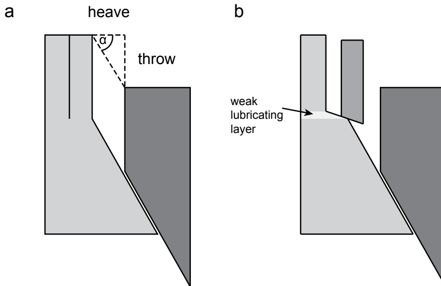
Figure 12. (a) Geometric relation between heave, throw and fault dip. (b) Lubricating layer can cause large blocks to break down.
