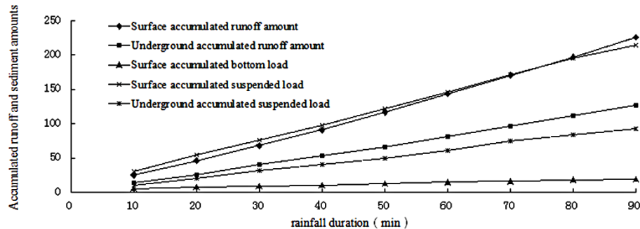
Figure 3. Variation of runoff and sediment production with rainfall duration under 30 % in pore fissure degree, degrees of holes and fissures with 3 %, bedrock rate with 50 \text{ mm h}^{-1} and 25^\circ in slope.
