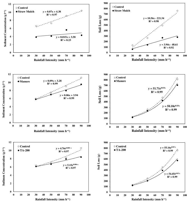
Figure 3. Relationships between rainfall intensity and organic and inorganic treatments on average sediment concentration (left column), soil loss (right column), rice straw mulch (top), manure (middle) and TA-200 polyacrylamide (bottom).
