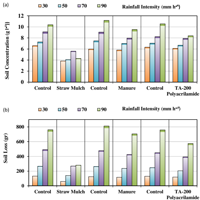
Figure 2. Average sediment concentration (a) and soil loss (b) at four rainfall intensities.
