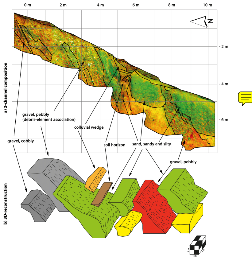
Figure 8. Results from the trenching site of Kokkalas et al. (2007). (a) 2-channel composition from multispectral approach. Red and green are 100 % different whereas yellow colouring represents intermediate correspondence of both channels. The trench log (black lines) fits with the multispectral cluster of a certain composition. (b) Three-dimensional reconstruction of the trench exposure. Recorded thickness of the colluvial wedge from 1981 is about 0.6 m.
