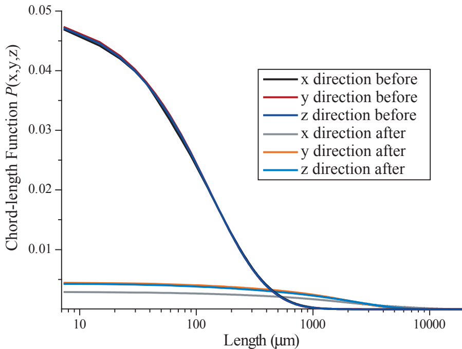
Figure 8. Chord length function along x , y and z ( P(x,y,z) ) for sample Bvl before and after the dissolution experiment.
