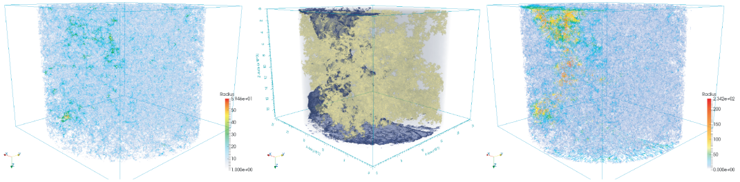
Figure 5. From left to right: extracted skeleton on sample Bvl_{be} , the formed wormholed in sample Bvl_{af} (blue) replaced in sample Bvl_{be} where the resolved connected porosity appears in yellow, extracted skeleton on sample Bvl_{af} . For the extracted skeleton images, the blue to red scale colors corresponds to pore size increase indicated in pixels (up to 60 pxls for sample Bvl_{be} and 234 pxls for sample Bvl_{af} ).
