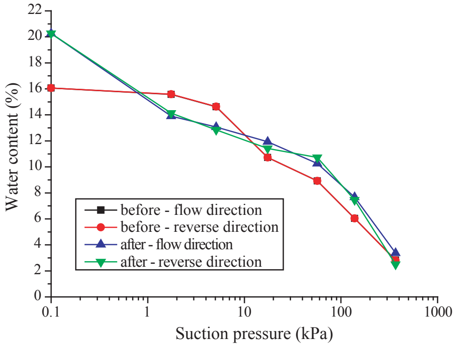
Figure 2. Retention curves before and after the dissolution experiment for sample Bvl.
