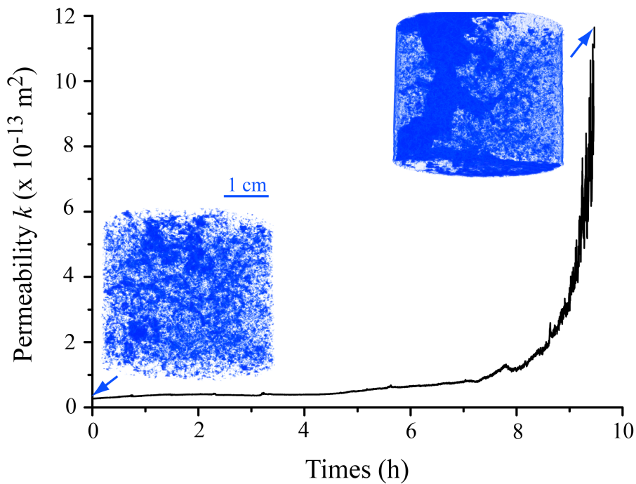
Figure 6. Time evolution of permeability k during dissolution experiment of sample Bvl. The corresponding 3-D images of the resolved porosity for sample Bvl be and Bvl af are reported for the initial and final percolation times.
