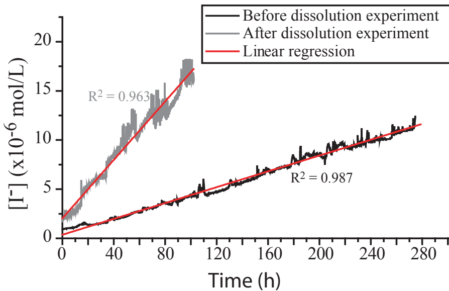
Figure 4. Iodine concentration measured in the sink cell during diffusion experiment through sample BvI before and after the dissolution experiment.
