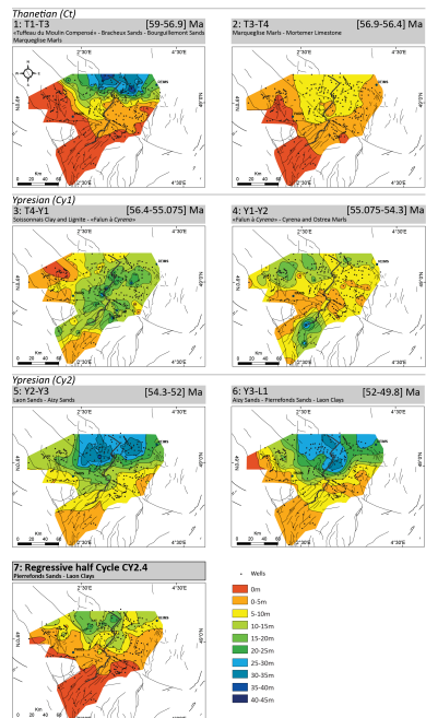
Figure 9. Isopach (sediment thickness) maps for each transgressive or regressive hemicycle of the three third-order cycles: Thanetian (Ct), Ypresian 1 (Cy1), Ypresian 2 (Cy2) and for the last fourth-order cycle of the regressive trend of Cy2 illustrating the erosion during the Late Ypresian unconformity.
