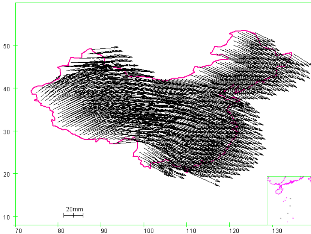
Fig. 1. 1^\circ \times 1^\circ Velocity Field Model
