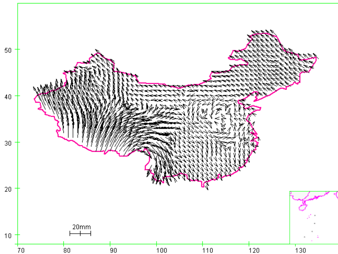
Fig. 2. 1^{\circ} \times 1^{\circ} Velocity Field Model deducing the Chinese continental crustal deformation background field
