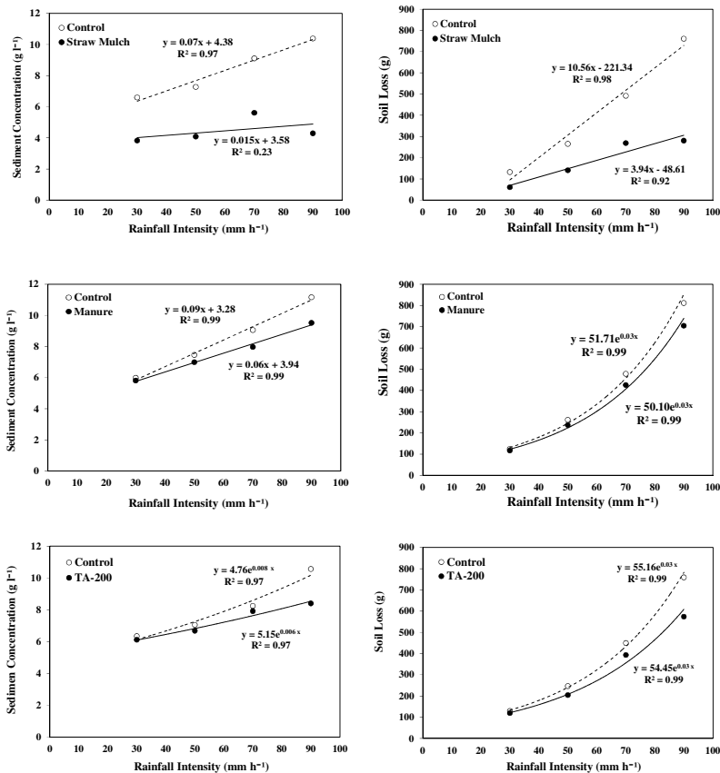
Figure 9. Relationships between rainfall intensity and organic and inorganic treatments on average sediment concentration (left column), soil loss (right column), rice straw mulch (top), manure (middle) and TA-200 polyacrylamide (bottom).
