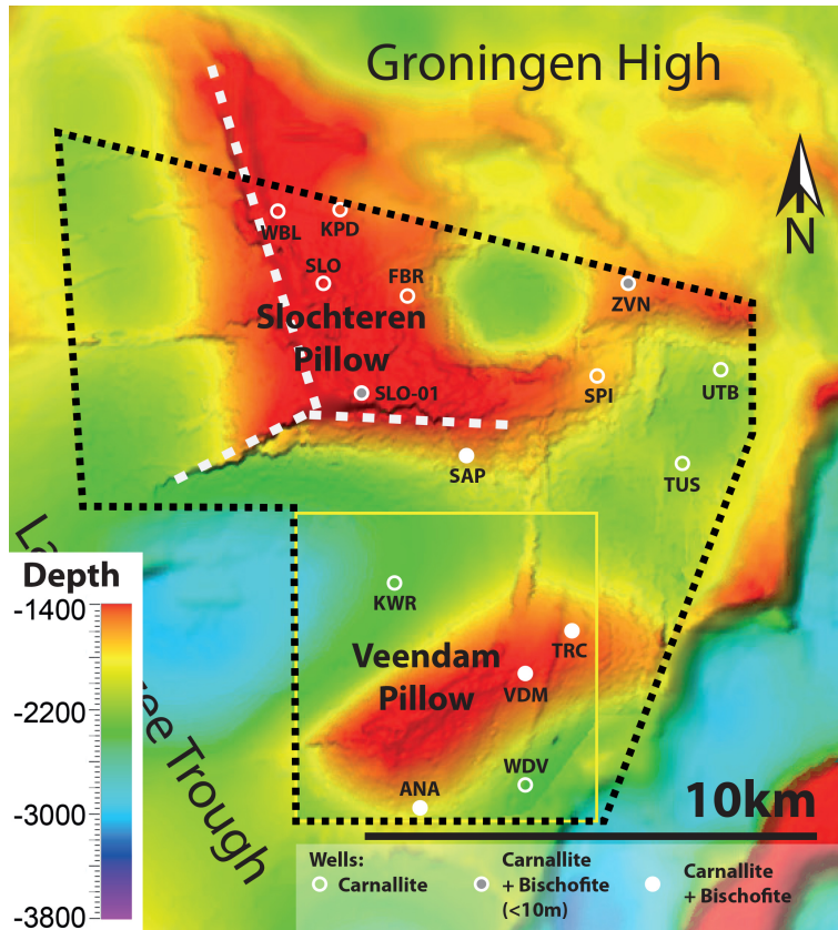
Figure 4. Top Salt surface map compiled after Strozyk et al. (2014) and this study, with well head locations. White dotted lines indicate major suprasalt faults at the Slochteren Pillow. The yellow box indicates the location of seismic volume 1.
