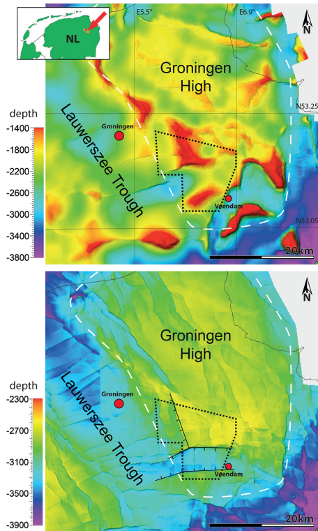
Figure 1. Top: Top salt map from the Groningen High (outline marked by with dotted line) and surrounding areas (modified after Strozyk et al., 2014). The dotted line indicates the outlines of 3-D seismic volumes covering the study area; Bottom: Base salt map from the Groningen High and surrounding areas (modified after Strozyk et al., 2014). Major normal faults (offset < 100 m) in the study area are marked.
