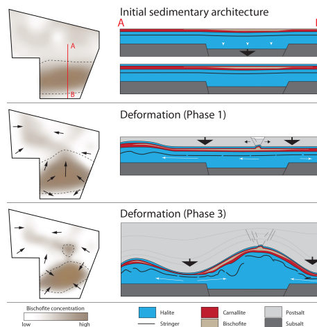
Figure 8. Conceptual reconstruction of salt deformation in the study area. The maps on the left side indicate movements in the bischofite deposit; the profile sketches ( a , b ) on the right side indicate corresponding deformation of the Zechstein (incl. ZIII stringer and K-Mg salts) and the suprasalt sediments. Black arrows indicate movements in the suprasalt sediments (e.g., extension and subsidence), white lines movements in the salt (e.g. salt withdrawal below sediment basins): (a) tectonic movements in the subsalt allow for localized bischofite deposition in the area of the later Veendam Pillow; (b) differential loading and extension in the Triassic sediments cause salt withdrawal and boudinage of the ZIII stringer in the area of the later Veendam Pillow, while salt accumulation and doming farther north triggers the formation of the Slochteren Pillow; K-Mg salts are initially deformed by extensional features in the salt’s overburden; (c) ongoing subsidence and salt withdrawal below sedimentary basins cause the formation of the Veendam Pillow and further grow of the Slochteren Pillow. The bischofite deposits are dragged into the Veendam Pillow, where they deform due to ZIII stringer deformation and structures in the supra-salt.
