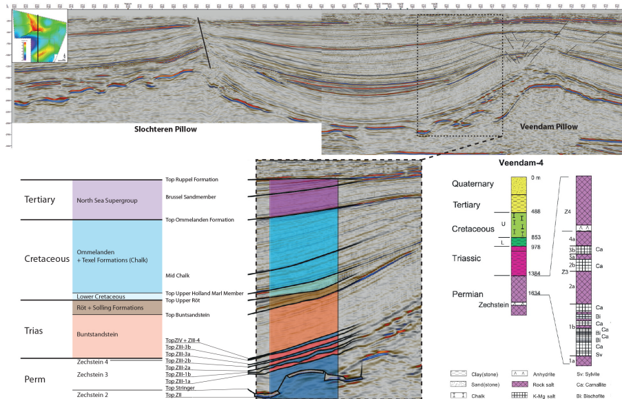
Figure 2. Top: N–S profile through the study area with the Slochteren Pillow in the north (volume 2) and the Veendam Pillow in the south (volume 1). The black lines indicate a normal fault at the south margin of the Slochteren Pillow and smaller faults above the Veendam Pillow forming a crestral collapse graben. The minibasin between the pillows shows significant thickening of most layers. The Z3 stringer is separated under the basin and folded and thrust in the pillows. Bottom: Detailed view of interpreted stratigraphic layers and units from the Veendam Pillow and Stratigraphy of the Veendam-4 well representative for the study area (modified after Geluk et al., 2007).
