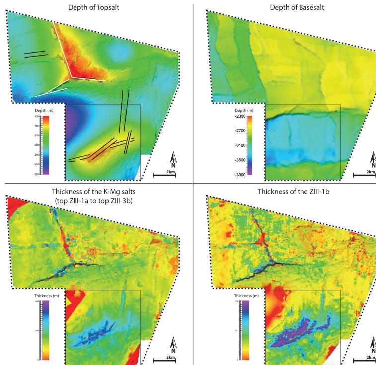
Figure 6. Detailed Top Salt map (black box indicates location of seismic volume 1) with surface inquiries (black lines) as a result of crestal collapses above salt pillows. The white lines indicate faults offsetting the Top Salt contact at the Slochteren Pillow. Thickness maps of top ZIII-1a to top ZIII-3b and top ZIII-1a to top ZIII-1b and a detailed map of the Subsalt surface (modified after Stroyk, 2014). Layers show significant thickening to the crest and under crestal collapse structures.
