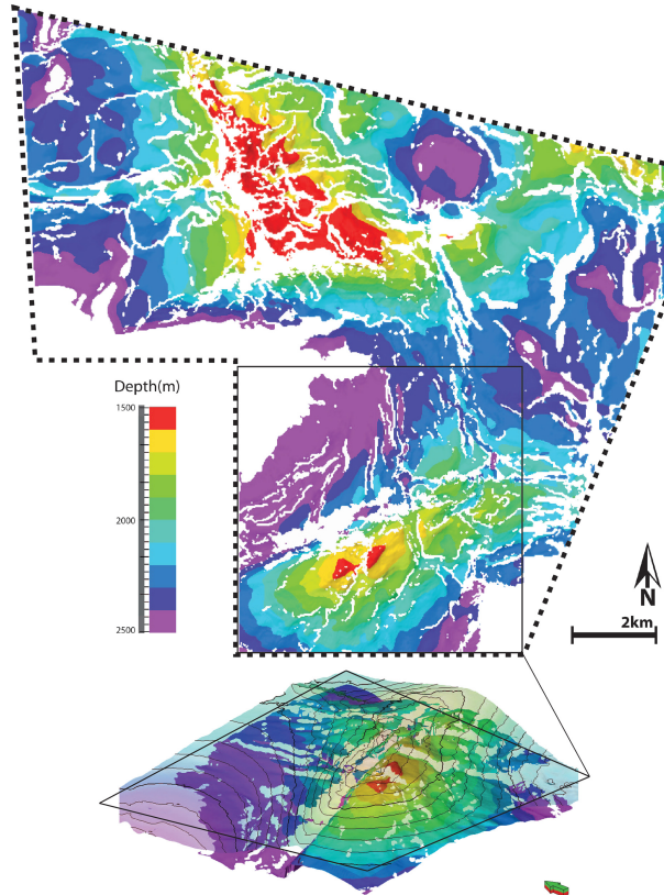
Figure 7. Map view of the ZIII stringer showing the different rupture patterns in the two pillows. The bird eyes view of the Veendam Pillow additionally shows the Topsalt surface. Here a deep stringer syncline in the NW of the Pillow is visible.
