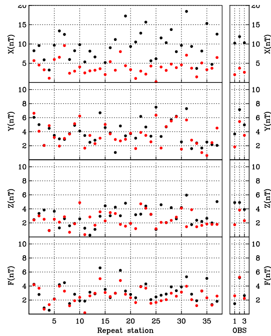
Figure 1. Standard deviation of individual repeat station (left) and observatory (right) lithospheric anomaly estimates around the mean value for southern Africa when only core field model values (black) or core and magnetospheric field model values (red) have been subtracted. In a few cases the difference is so small that the black dot is hidden behind the red one.
