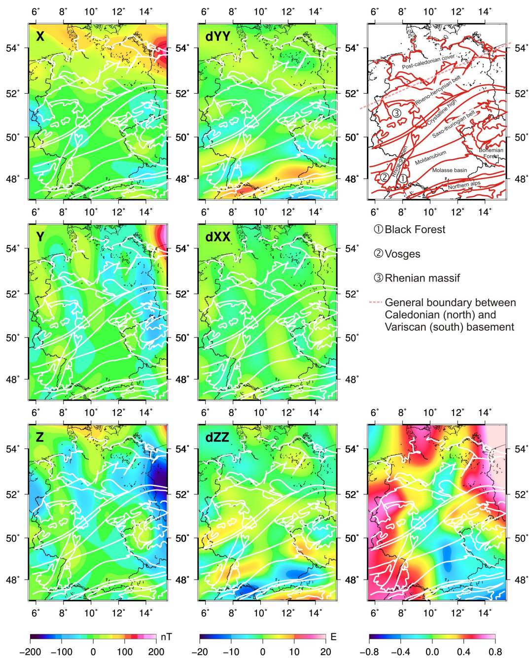
Figure 9. Comparison of long-wavelength magnetic and gravity anomalies for Germany. Left: Lithospheric field from EMM2010 model of SH degrees 15-200 for X-north (top X) , Y-east (middle Y) and Z-vertical (bottom Z) component components from top to bottom. Middle: Gravity gradients in north ( top dYY ), east ( middle dXX ) and vertical ( bottom dZZ ) direction-directions from top to bottom from GOCE-DIR5 model up to SH degree 200. Right: Labelled outline of large-scale tectonic features (top) after Berthelsen et al. (1992) and correlation between vertical component magnetic and gravity anomalies (bottom).
