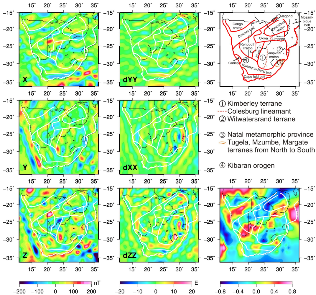
Figure 8. Comparison of long-wavelength magnetic and gravity anomalies for the southern African region. Left: Lithospheric field from EMM2010 model of SH degrees 15-200 for X-north (top X ), Y-east (middle Y ) and Z-vertical (bottom Z ) componentcomponents from top to bottom. Middle: Gravity gradients in north (top dYY ), east (middle dXX ) and vertical (bottom dZZ ) direction-directions from top to bottom from GOCE-DIR5 model up to SH degree 200. Right: Labelled outline of large-scale tectonic features (top) after Thomas et al. (1993) and Webb (2009) and correlation between vertical component magnetic and gravity anomalies (bottom).
