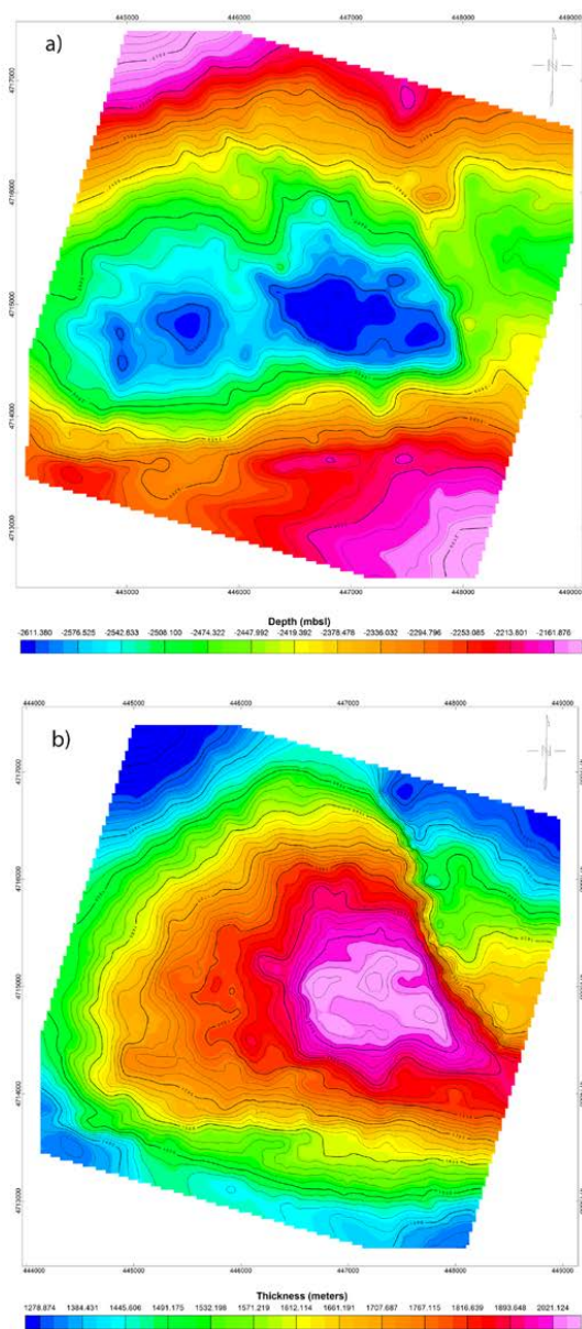
Figure 7: a) Basement topography derived from inversion of the residual gravity data shown in figure 6d and b) thickness map of the Triassic Keuper evaporites after comparing the basement topography and the bottom of the sedimentary sequence
