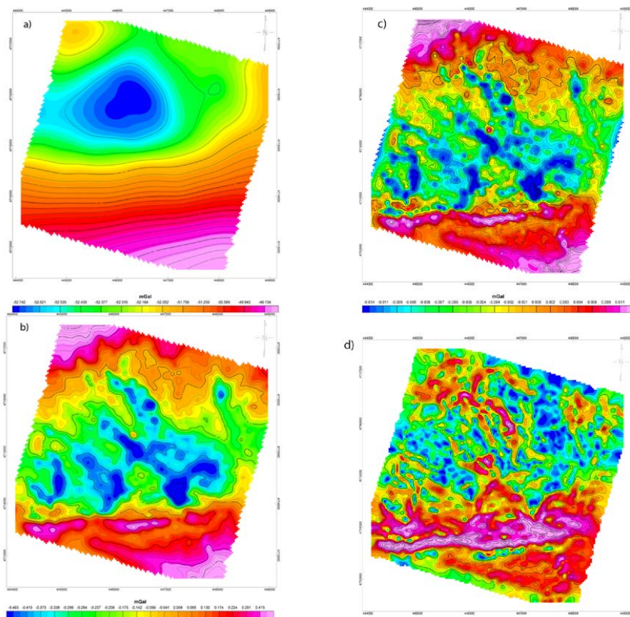
Figure 4: a) Regional gravity anomaly of the study area obtained by upward continuation up to 350 m, b) resulting residual anomaly, c) first vertical derivative of the Bouguer Anomaly (BA) map (order 0.75), d) total horizontal derivative (THD) of the BA map
