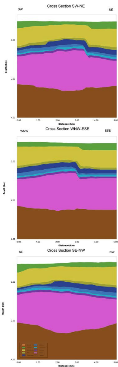
Figure 5d: Cross section extracted from the 3D gravity model of the basement (Figure 7a) generated integrating 3D seismics and microgravity inversion results (see figure 3 for location).
