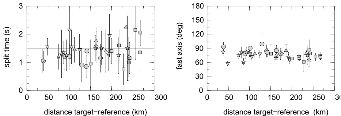
Fig. 2. Plot of splitting parameters ( \varphi and \delta t ) as a function of inter-station spacing of the target and reference station for a particular event C101703B, CMT ID (-05.47°, +154.15°) which recorded at target
