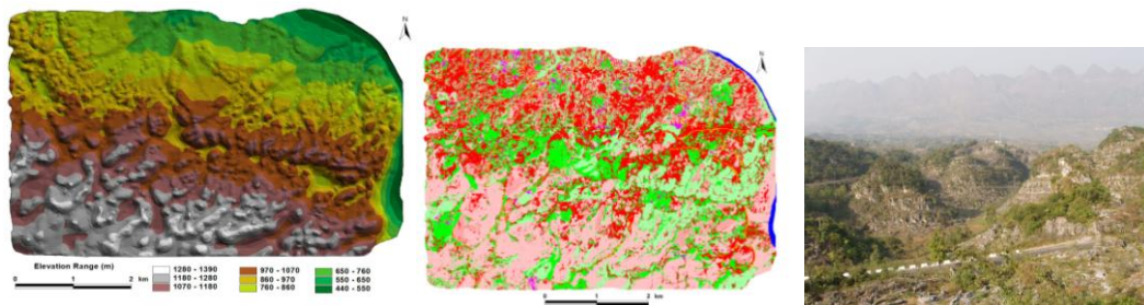
Peak cluster-canyon
