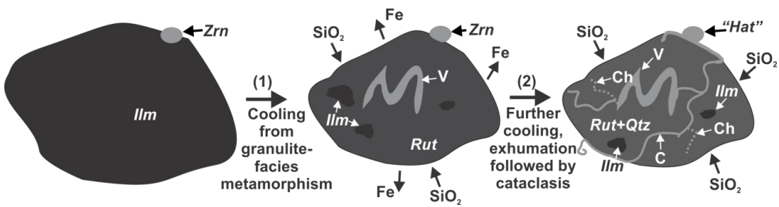
Figure 6: Schematic sketch of the formation stages of zircon coronas. (1) Pre-existing metamorphic Zr-bearing ilmenite starts decomposing to rutile and forms vermicular-shaped zircon aggregates or exsolution lamellae as a side product. The system loses Fe and requires SiO 2 from the surrounding phases, the volume of Fe-Ti oxide decreases. Round metamorphic zircon experiences slight dissolution where it's adjacent to ilmenite, which results in the final “hat” shape. This happens during and soon after granulite-facies peak metamorphism at the initial cooling stage. (2) Further cooling and exhumation results in re-crystallization of Zr-rich rutile with exsolution of thin zircon coronas, followed by cataclasis, crystal-plastic deformation and formation of rutile-quartz intergrowths. System requires SiO 2 from the environment. Abbreviations as in Figs. 1, 3 and 5.
