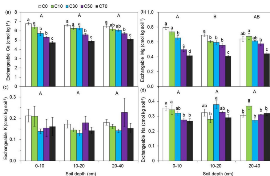
Fig. 2 Soil base cations of exchangeable Ca (a), Mg (b), K (c) and Na (d) for three soil 5 depths in different soil coarseness degrees of 0% sand addition (C0), 10% (C10), 30% (C30), 50% (C50) and 70% (C70). Data represent mean \pm SE (n=6). Letters indicate significant differences among treatments (lowercase letters) and differences among soil depths when averaging across all treatments (capital letters).
