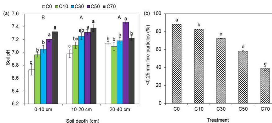
Fig. 1 Soil pH values for three soil depths (a) and proportion of soil fine particles (< 0.25 mm) for 0-10 cm soil in different soil coarseness degrees of 0% sand addition (C0), 10% (C10), 30% (C30), 50% (C50) and 70% (C70). Data represent mean \pm SE (n=6). Letters indicate significant differences among treatments (lowercase letters) and differences among soil depths when averaging across all treatments (capital letters).
