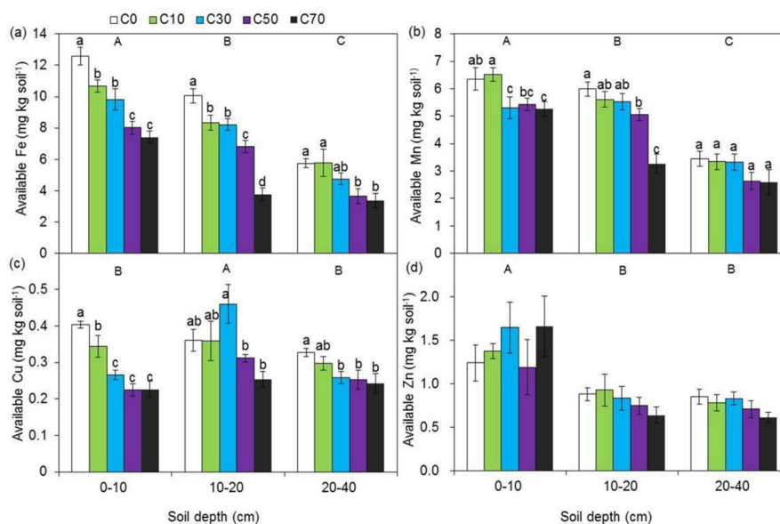
Fig. 3 Soil available micronutrients of available Fe(a), Mn (b), Cu (c) and Zn (d) for three soil depths in different soil coarseness degrees of 0% sand addition (C0), 10% (C10), 30% (C30), 50% (C50) and 70% (C70). Data represent mean \pm SE (n=6). Letters indicate significant differences among treatments (lowercase letters) and differences among soil depths when averaging across all treatments (capital letters).
