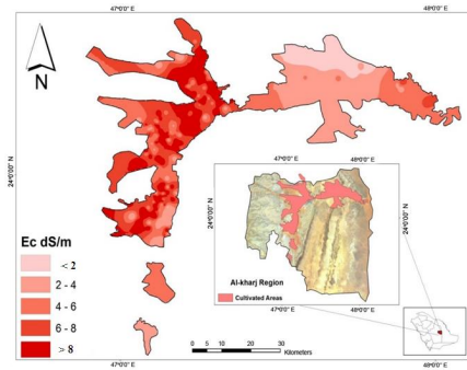
Figure 9. Interpolation of groundwater EC
