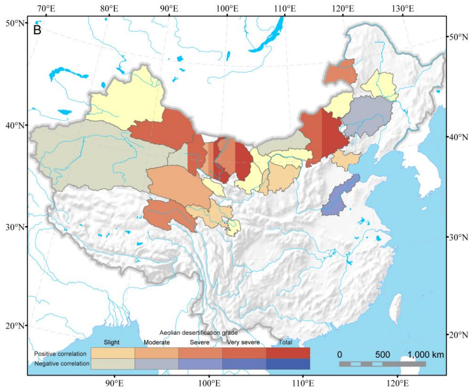
28 Figure S3. Relationships between the (a) NDVI and (b) VFC and trends in aeolian desertification.
