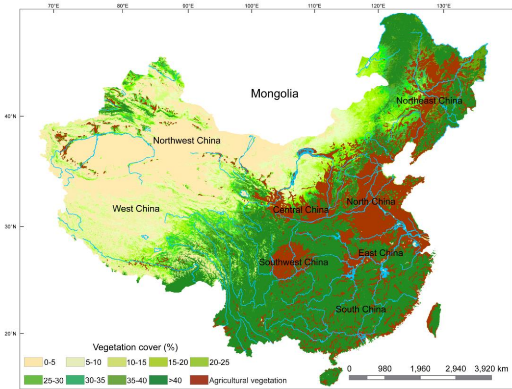
40 Figure S5. Vegetation cover and the major areas of agricultural activity in China.
