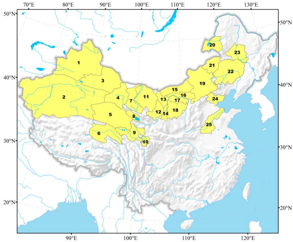
19 Figure S2. Areas monitored for aeolian desertification over the past decades in China.
