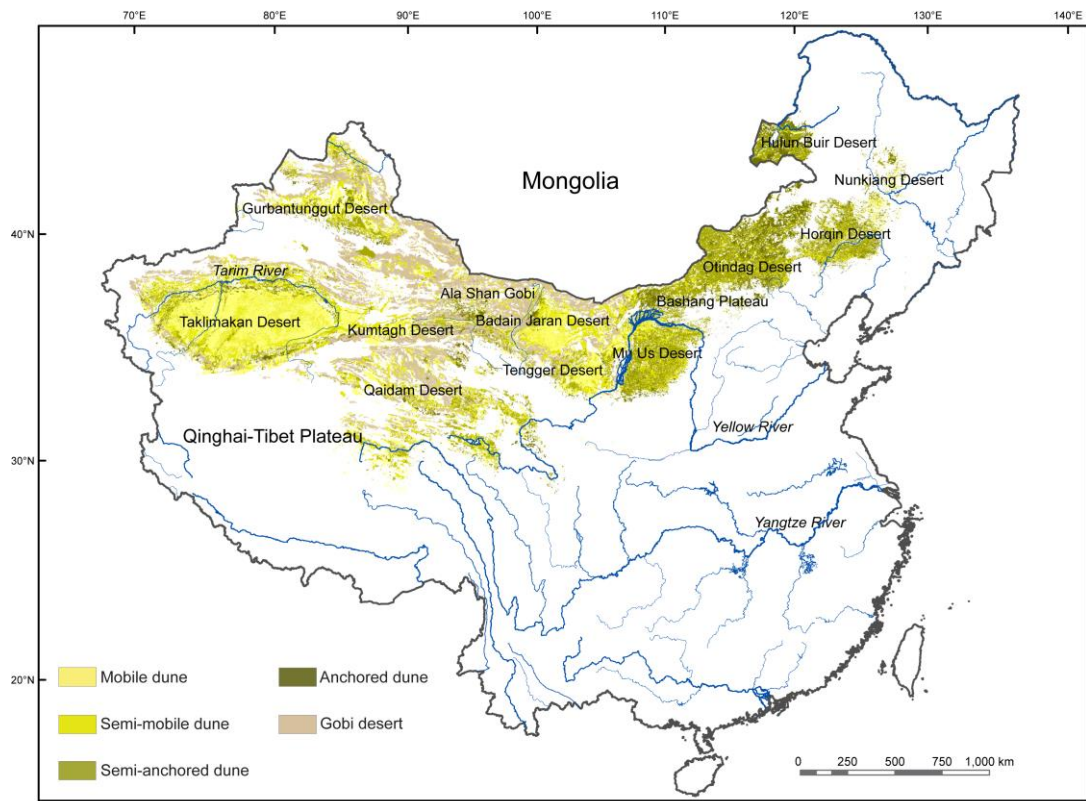
16 Figure S1. Distribution of the sandy and gobi deserts in China.
