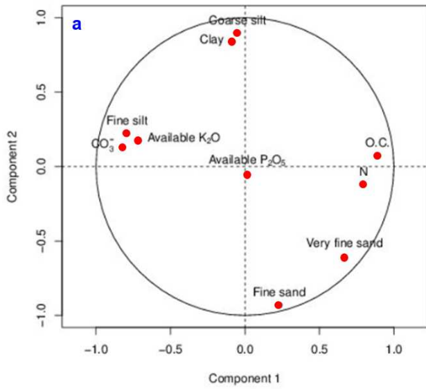
Figure 4. Plot of the correlation coefficients within a unit circle on the plane of Components 1 and 2 (a) and Components 1 and 3 (b).
