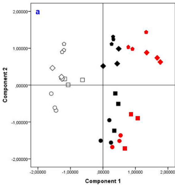
Figure 5. Scatter plot of the height-dust from Calcisols (CL), Cambisols (CM) and Luvisols (LV) categories for the Components 1 and 2 matrix (a) and the Components 1 and 3 matrix (b).
