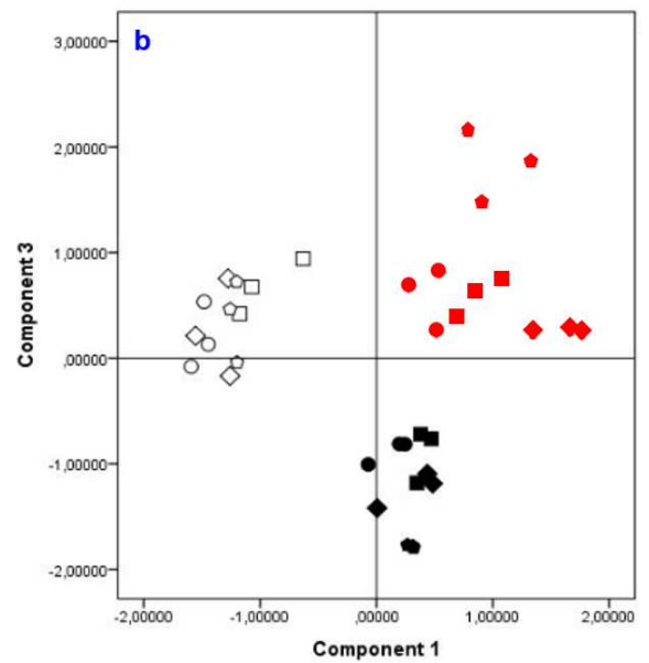
Figure 5. Scatter plot of the height-dust from Calcisols (CL), Cambisols (CM) and Luvisols (LV) categories for the Components 1 and 2 matrix (a) and the Components 1 and 3 matrix (b).
